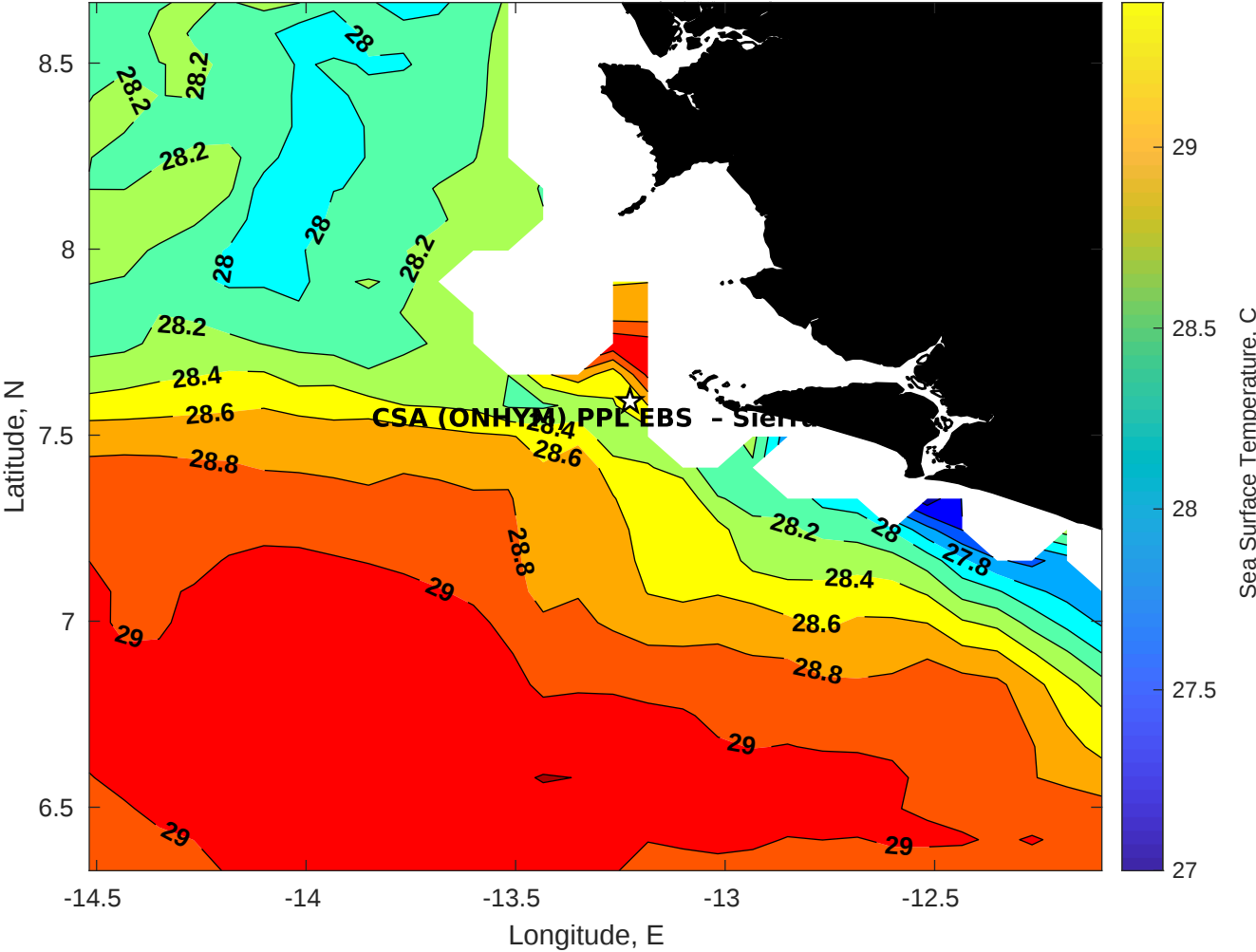
SST for CSA (ONHYM) PPL EBS - Sierra Leone at 28-Dec-2025 00:00:00
