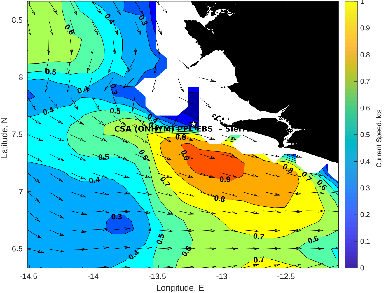
Surface Currents for CSA (ONHYM) PPL EBS - Sierra Leone at 28-Dec-2025 00:00:00
