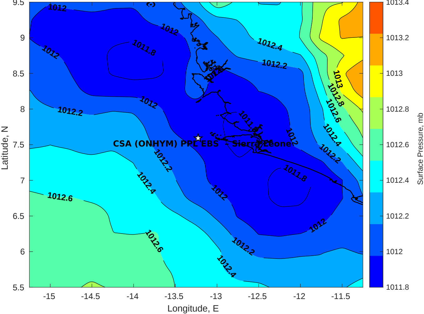
Surface Pressure (mb) for CSA (ONHYM) PPL EBS - Sierra Leone at 29-Dec-2025 00:00:00
