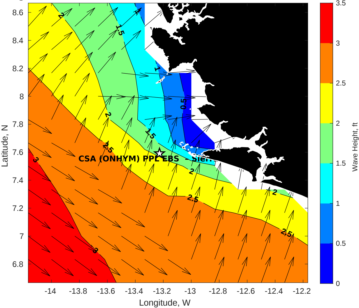
GFS Wave Height (ft) for CSA (ONHYM) PPL EBS - Sierra Leone at 29-Dec-2025 09:00:00
