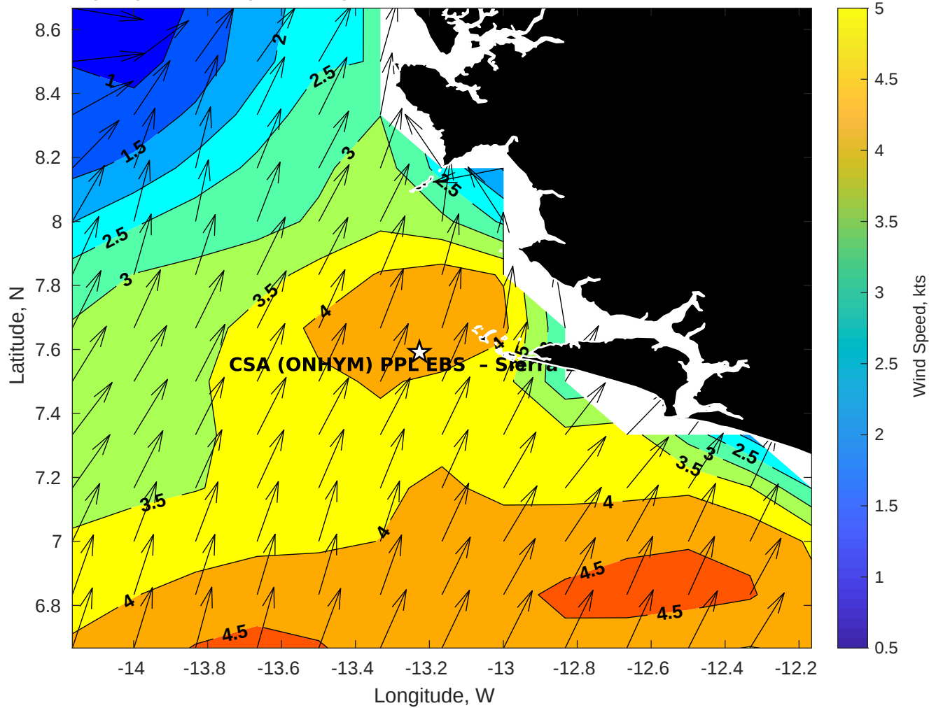
GFS Winds (kts) for CSA (ONHYM) PPL EBS - Sierra Leone at 29-Dec-2025 09:00:00
