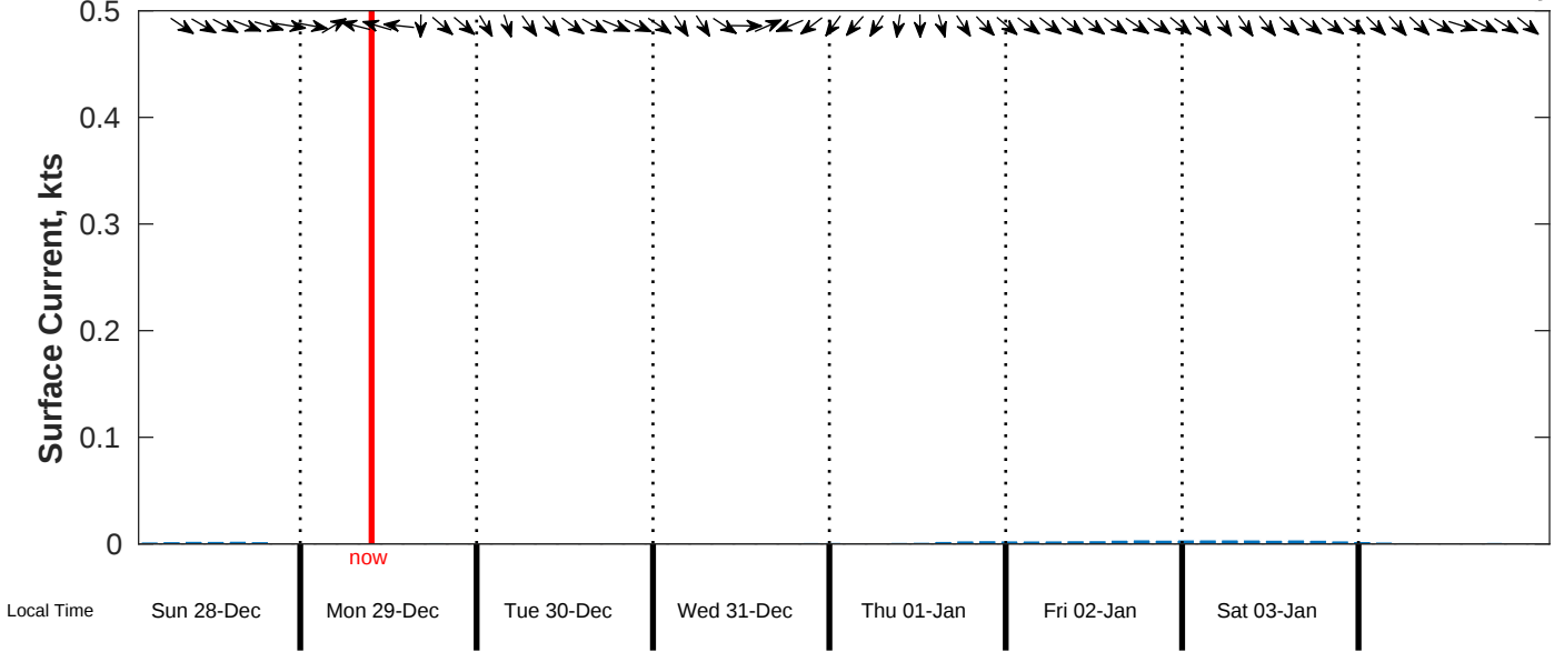
Surface Current Forecast for CSA (ONHYM) PPL EBS - Sierra Leone from 28-Dec-2025 00:00:00 to 05-Jan-2026 00:00:00
