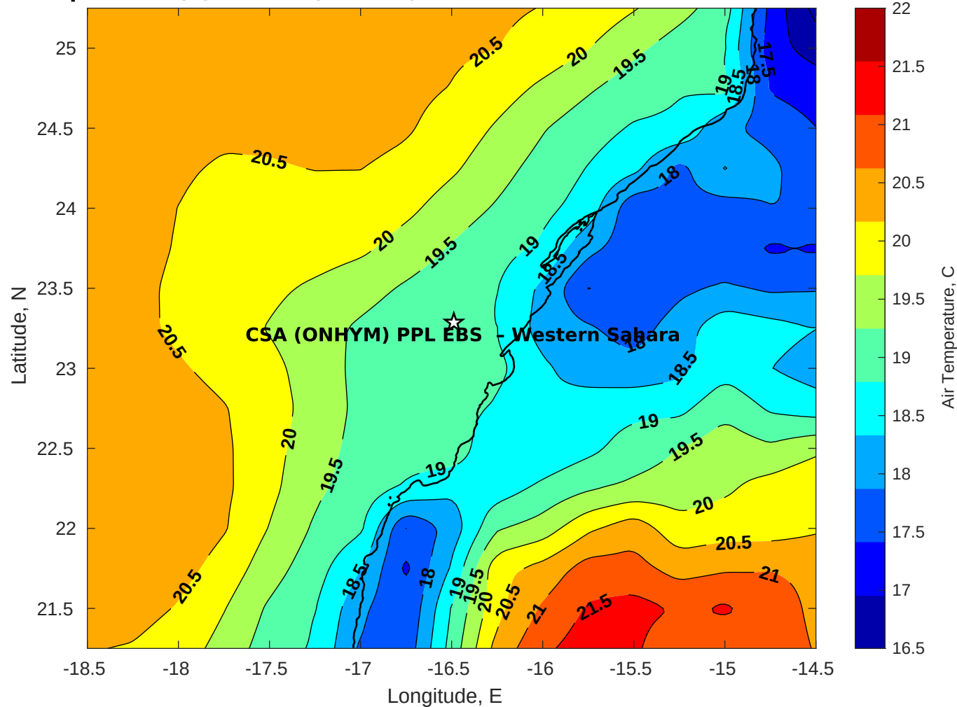
Air Temperature (C) for CSA (ONHYM) PPL EBS - Western Sahara at 29-Dec-2025
