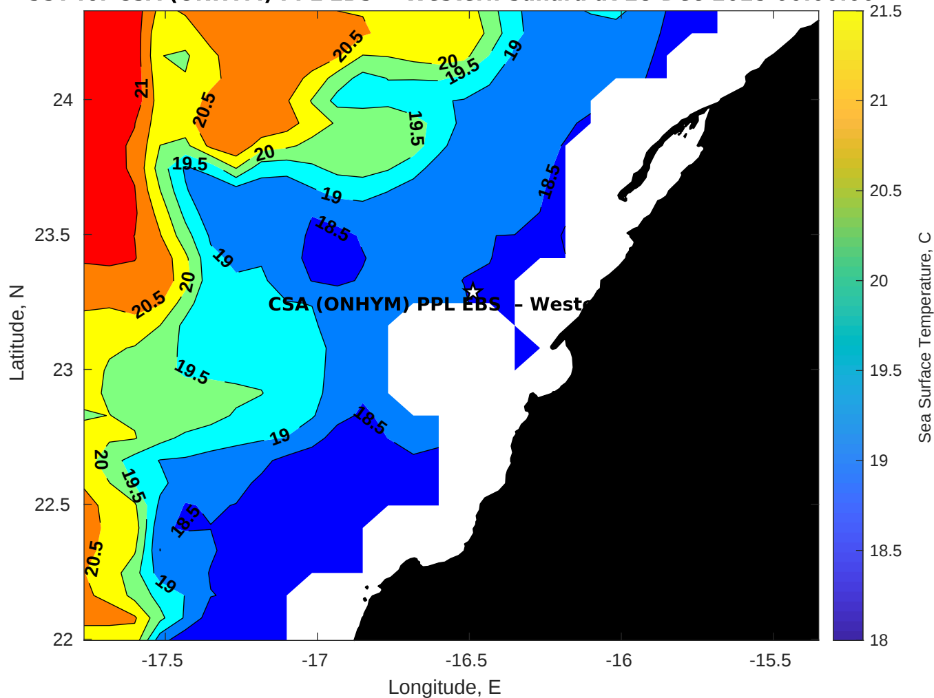
SST for CSA (ONHYM) PPL EBS - Western Sahara at 28-Dec-2025 00:00:00
