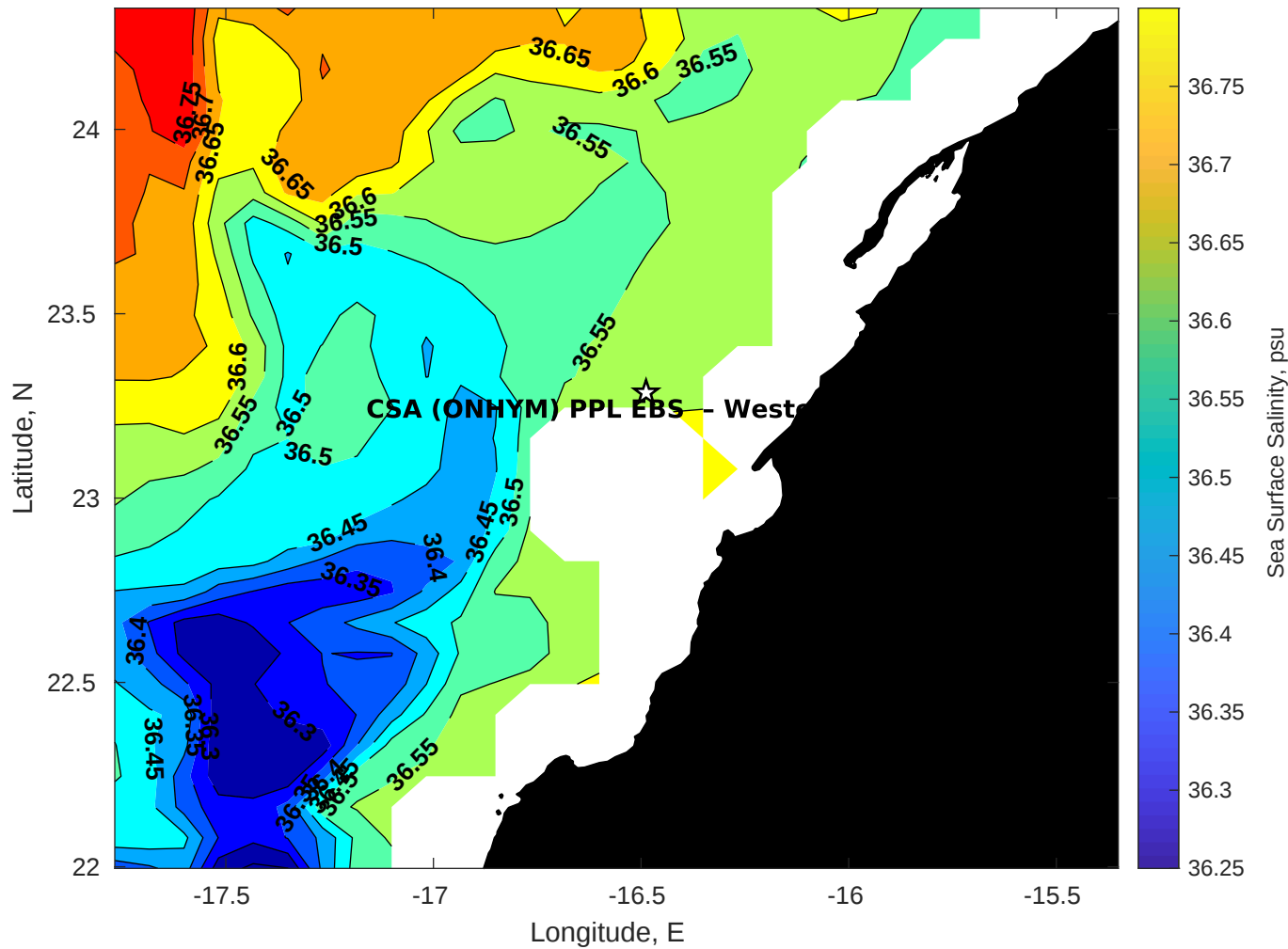
Surface Salinity for CSA (ONHYM) PPL EBS - Western Sahara at 28-Dec-2025 00:00:00
