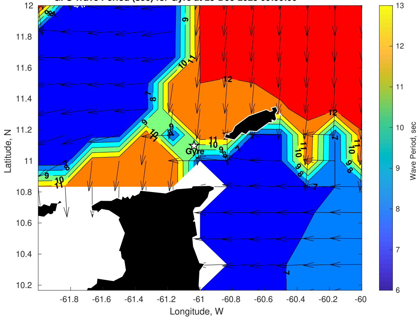
GFS Wave Period (sec) for Gyre at 29-Dec-2025 09:00:00
