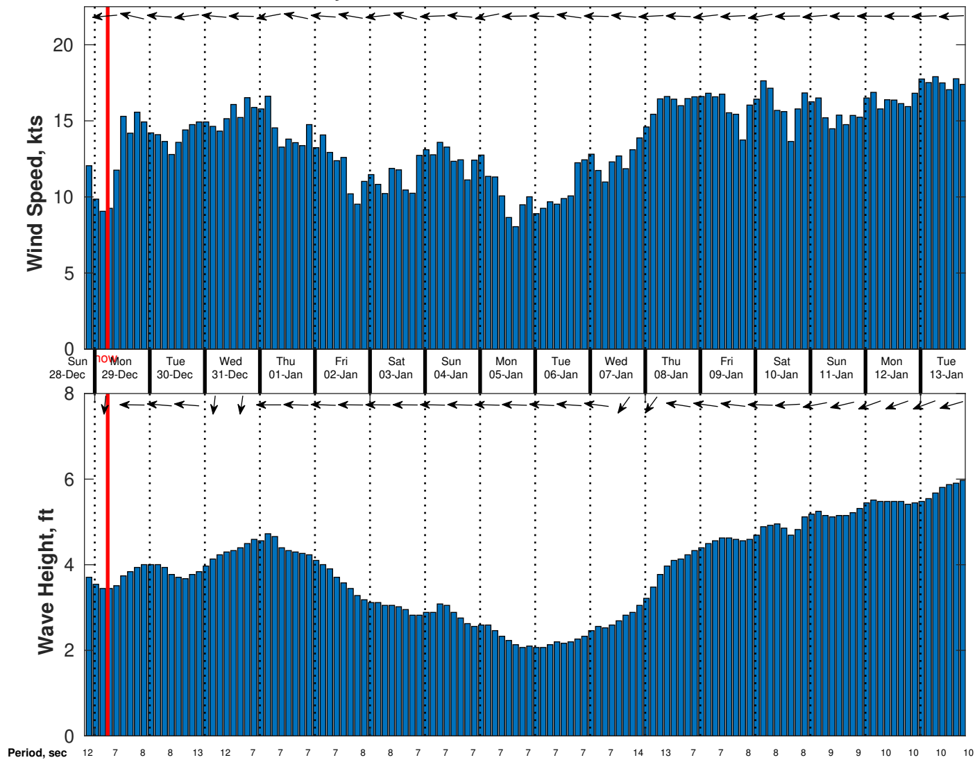
Wind & Wave Forecast for Gyre from 28-Dec-2025 20:00:00 to 13-Jan-2026 20:00:00
