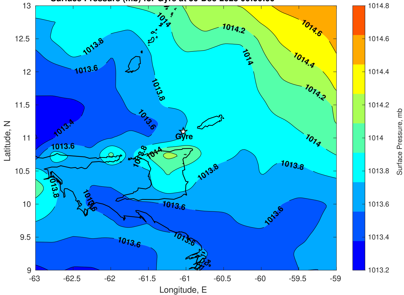
Surface Pressure (mb) for Gyre at 30-Dec-2025 00:00:00
