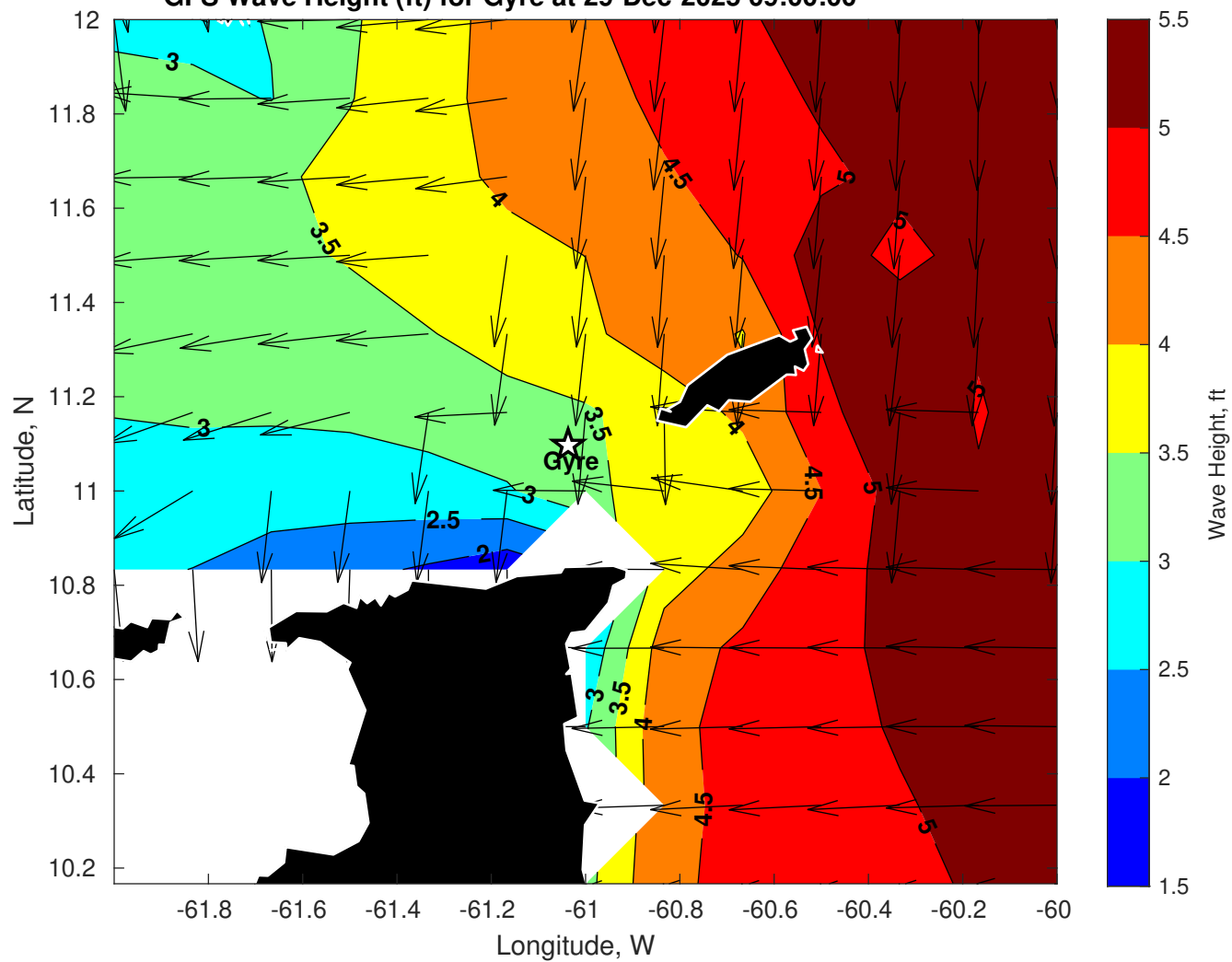
GFS Wave Height (ft) for Gyre at 29-Dec-2025 09:00:00
