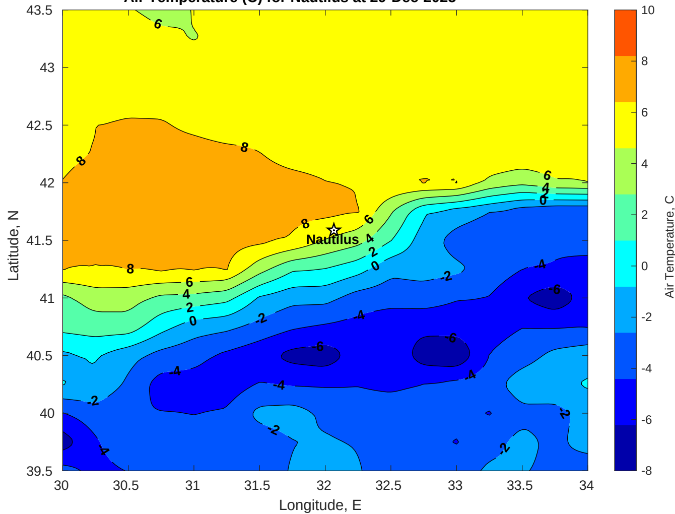
Air Temperature (C) for Nautilus at 29-Dec-2025
