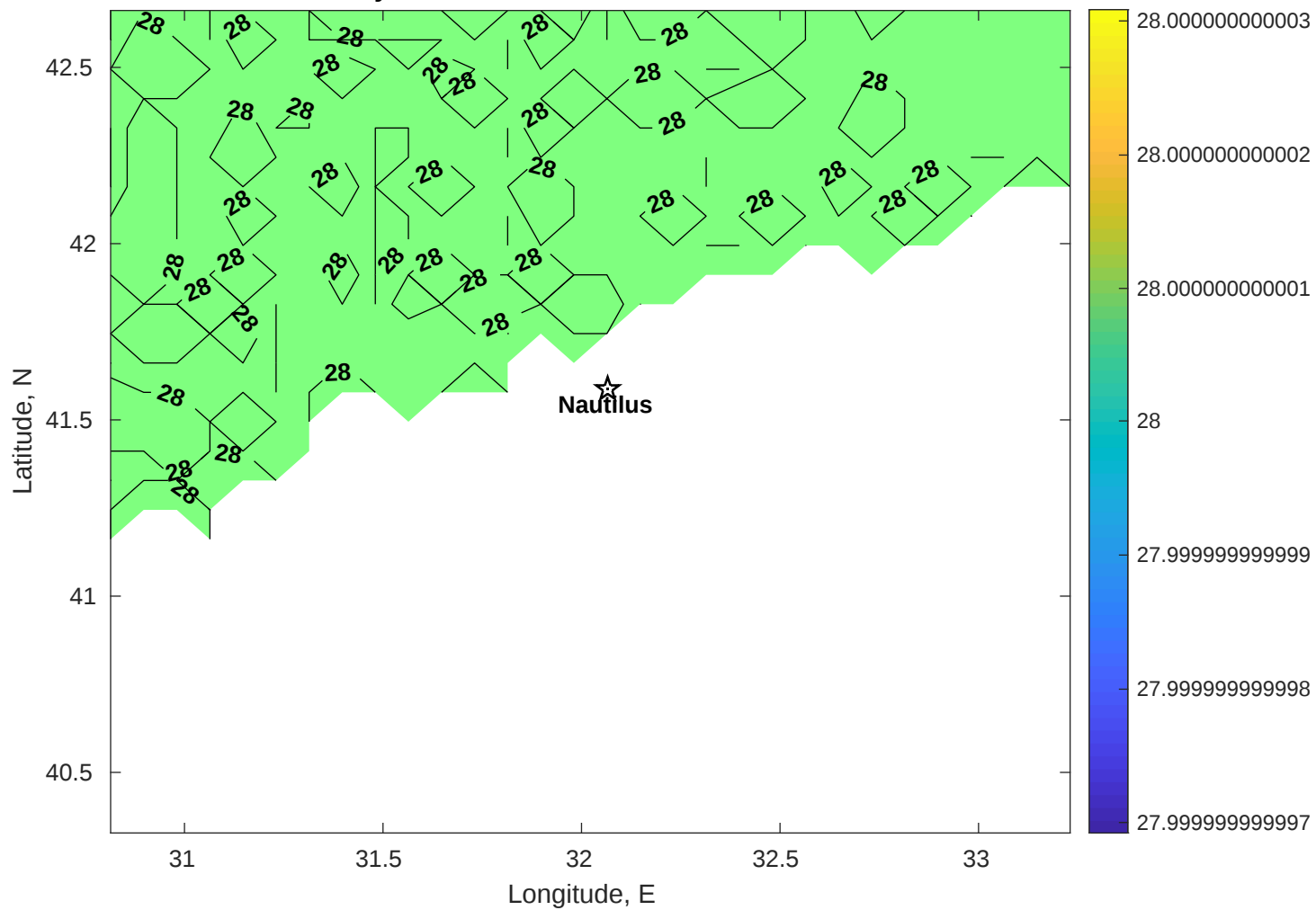
Surface Salinity for Nautilus at 28-Dec-2025 00:00:00
