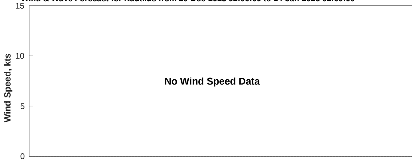
Wind & Wave Forecast for Nautilus from 29-Dec-2025 02:00:00 to 14-Jan-2026 02:00:00
