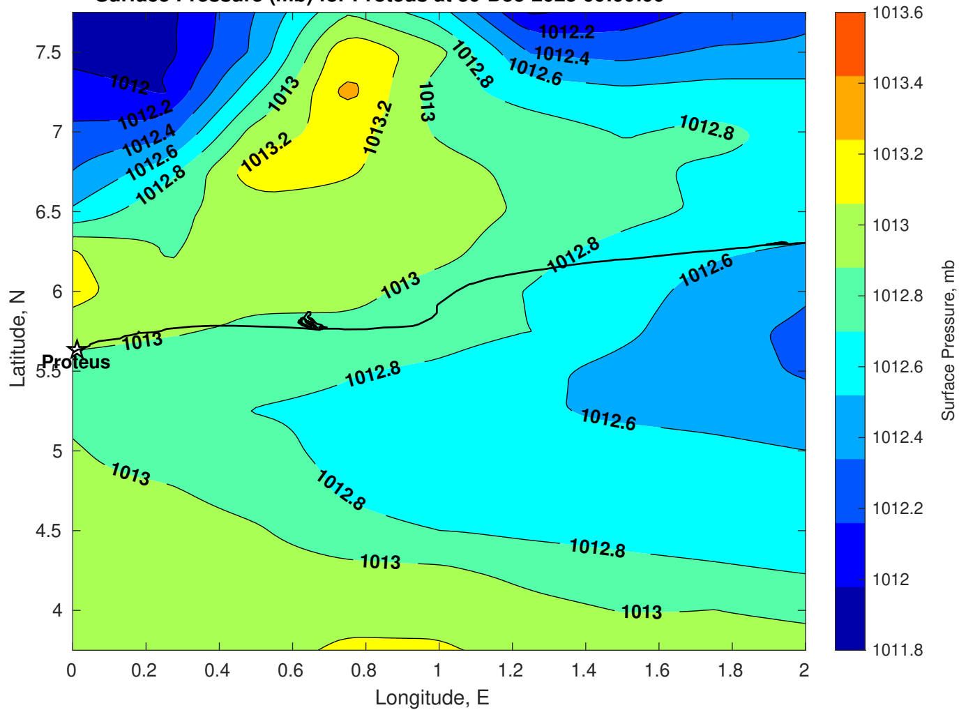
Surface Pressure (mb) for Proteus at 30-Dec-2025 00:00:00
