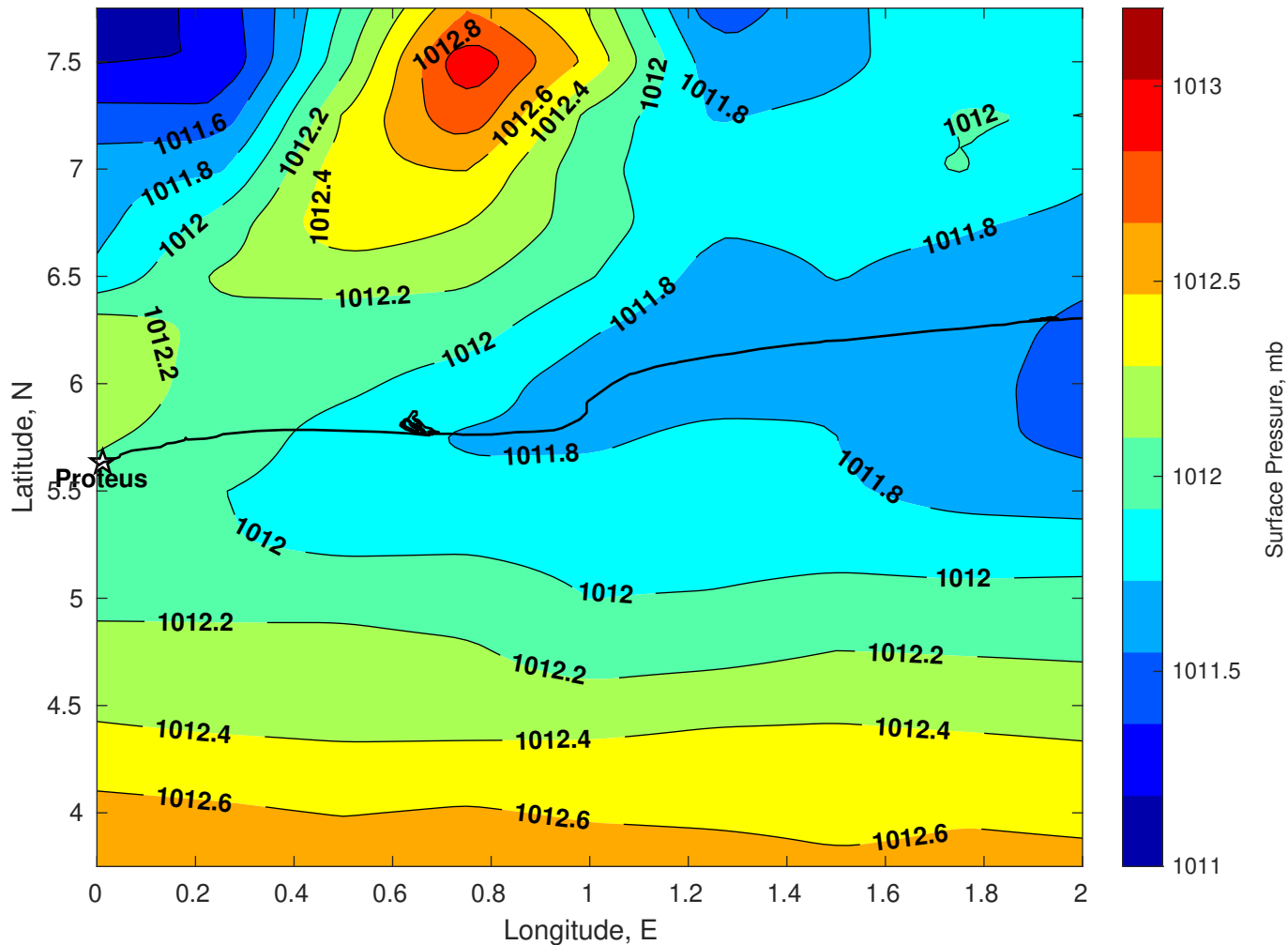
Surface Pressure (mb) for Proteus at 29-Dec-2025 00:00:00
