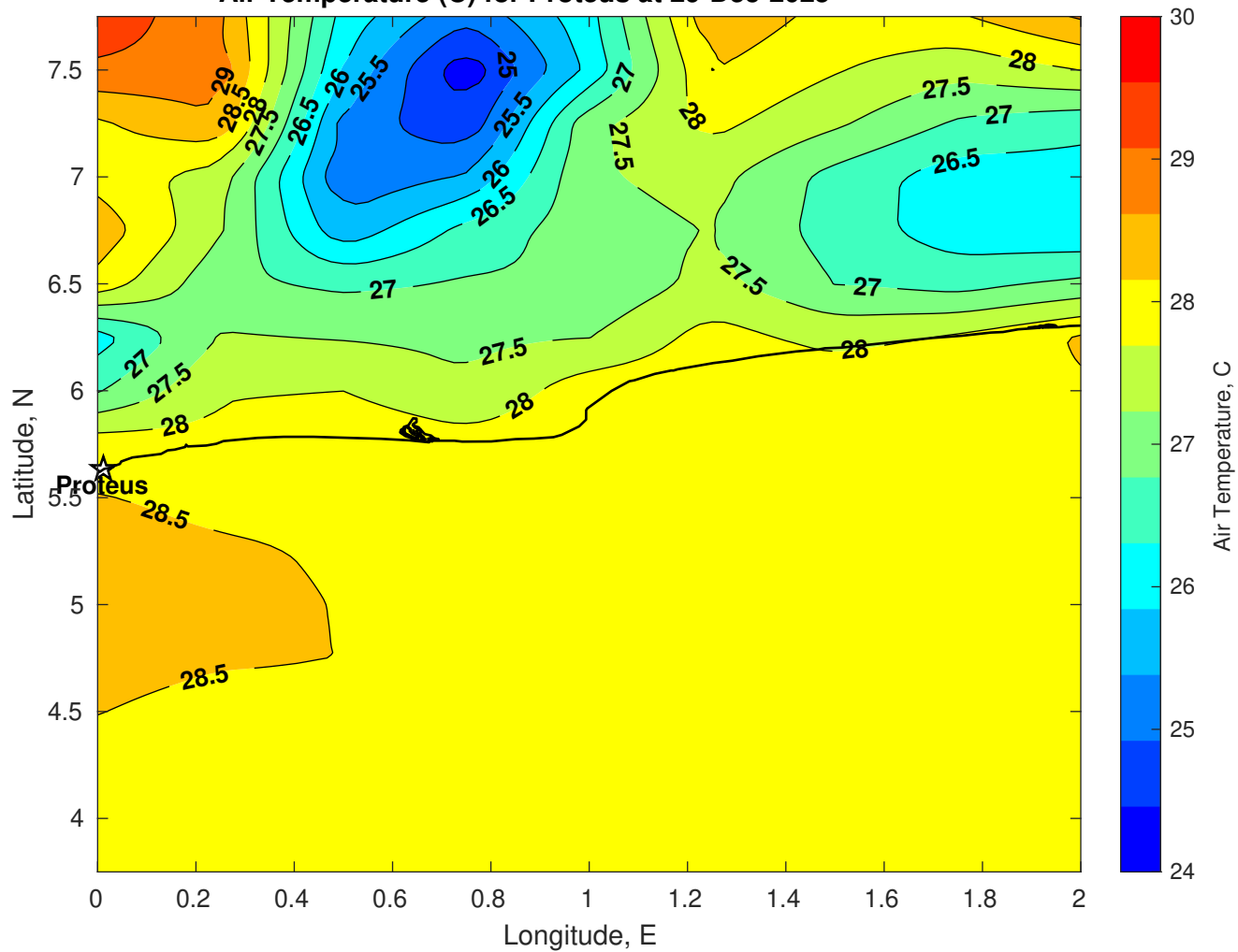
Air Temperature (C) for Proteus at 29-Dec-2025
