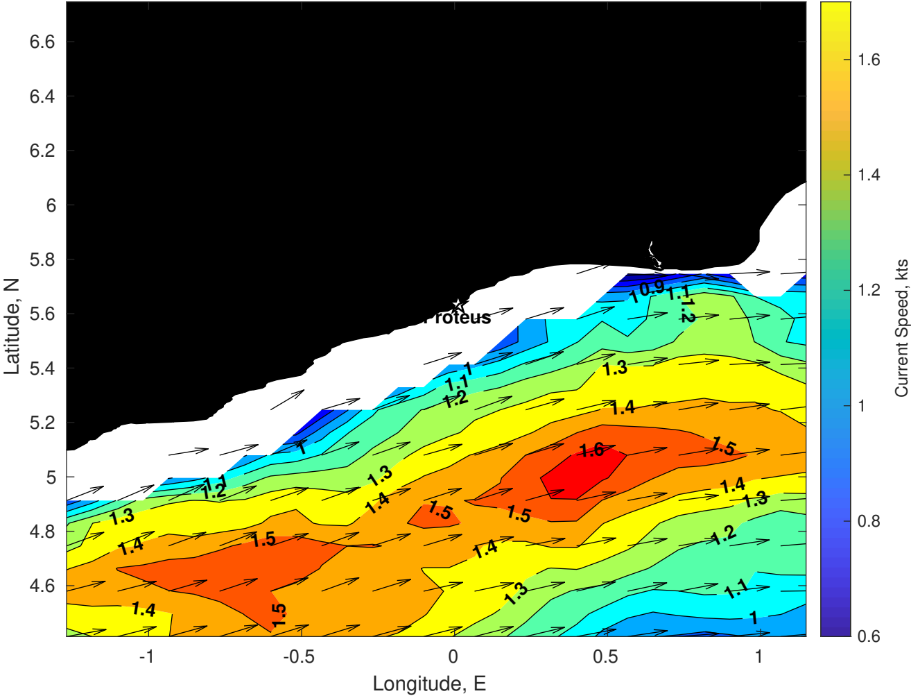
Surface Currents for Proteus at 28-Dec-2025 00:00:00
