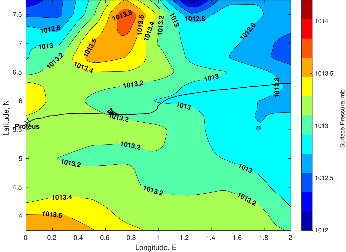
Surface Pressure (mb) for Proteus at 31-Dec-2025 00:00:00
