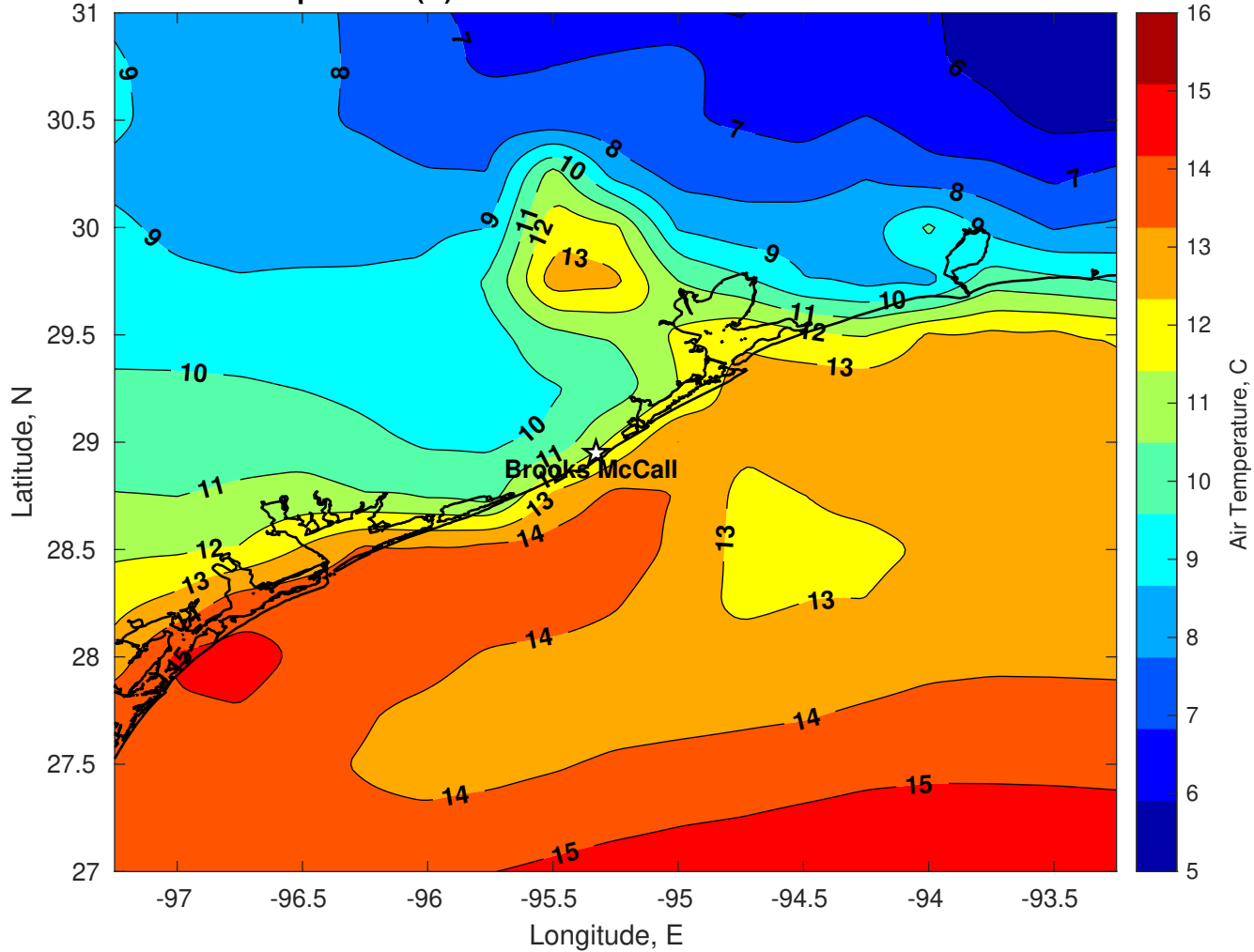
Air Temperature (C) for Brooks McCall at 30-Dec-2025
