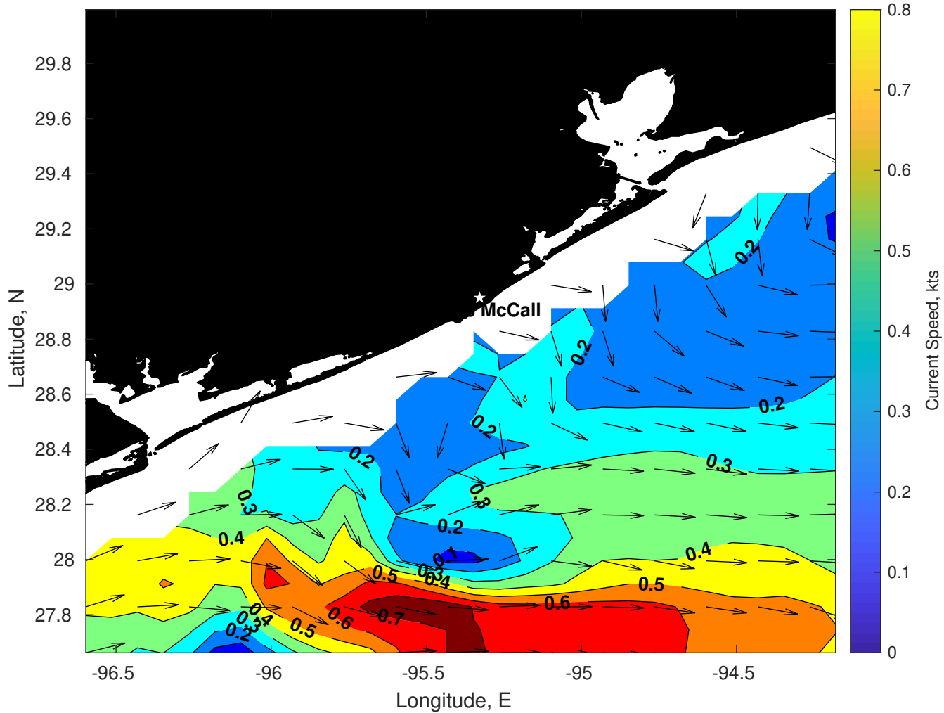
Surface Currents for Brooks McCall at 29-Dec-2025 00:00:00
