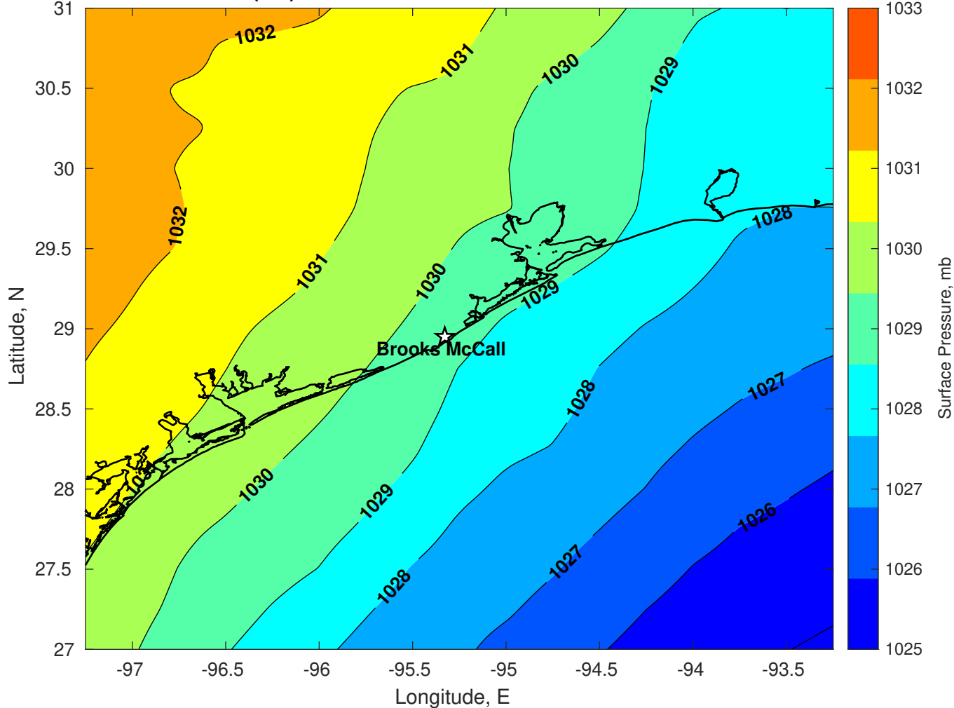
Surface Pressure (mb) for Brooks McCall at 30-Dec-2025 00:00:00
