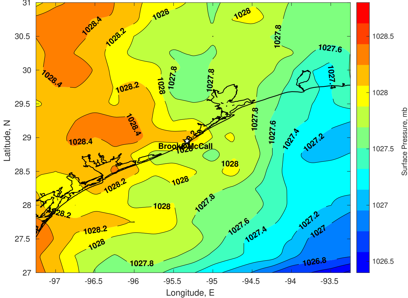
Surface Pressure (mb) for Brooks McCall at 31-Dec-2025 00:00:00
