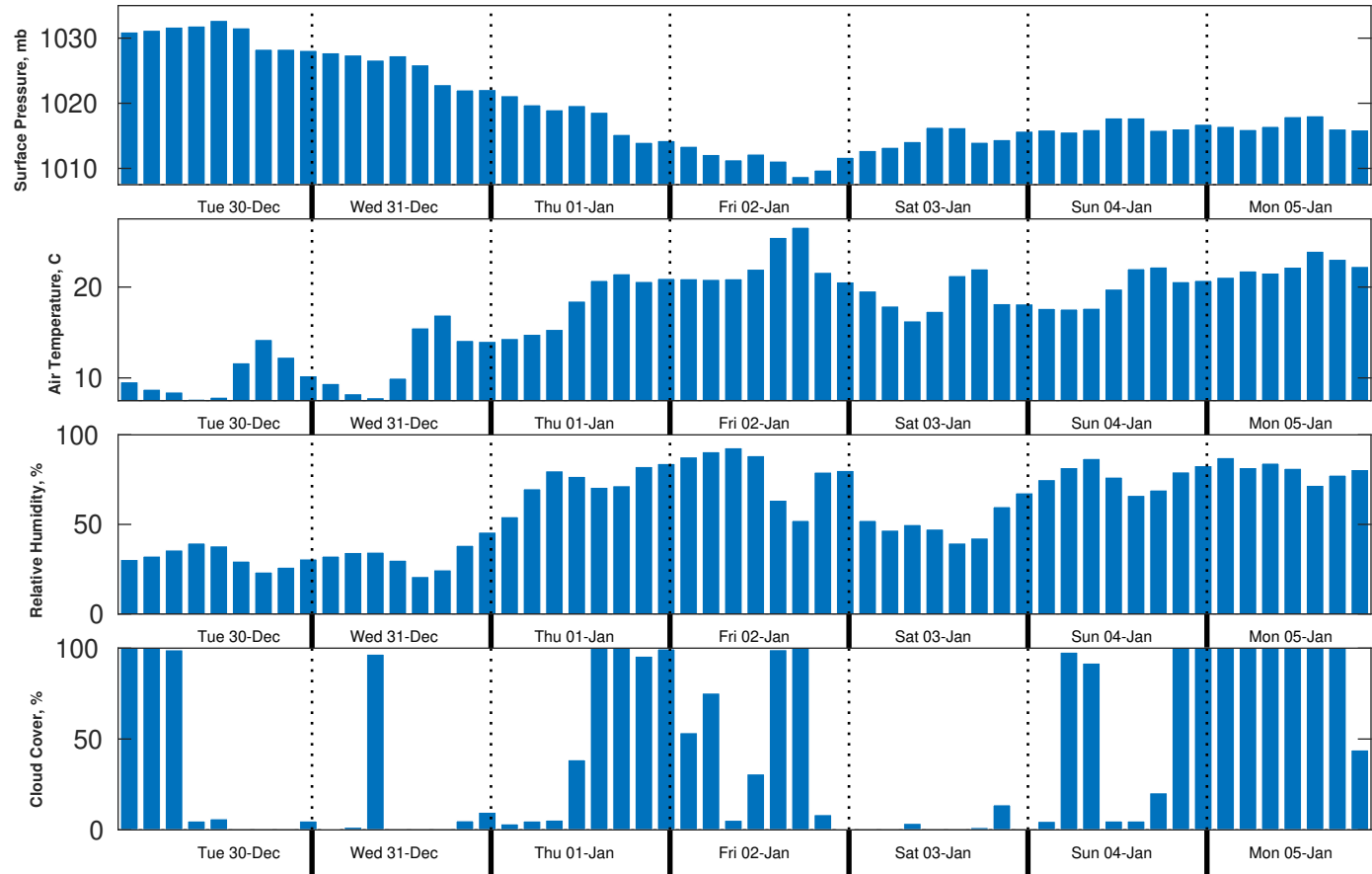
Met Forecast for Brooks McCall from 30-Dec-2025 00:00:00 to 06-Jan-2026 00:00:00
