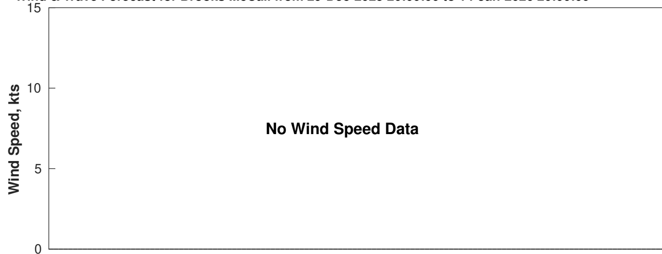
Wind & Wave Forecast for Brooks McCall from 29-Dec-2025 20:00:00 to 14-Jan-2026 20:00:00
