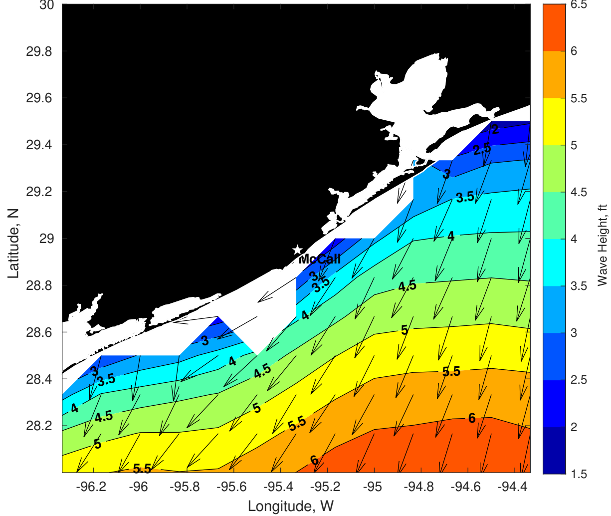
GFS Wave Height (ft) for Brooks McCall at 30-Dec-2025 09:00:00
