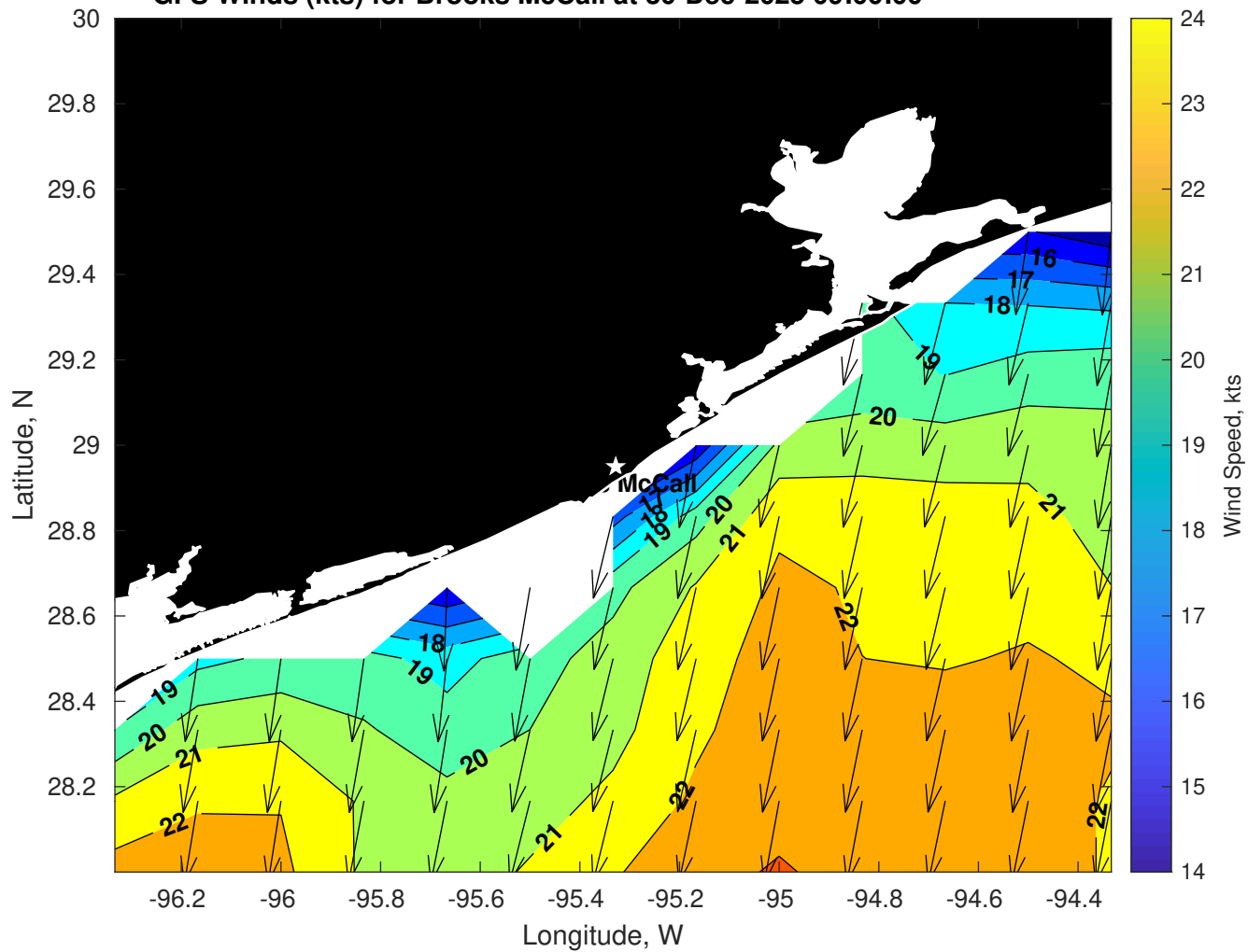
GFS Winds (kts) for Brooks McCall at 30-Dec-2025 09:00:00
