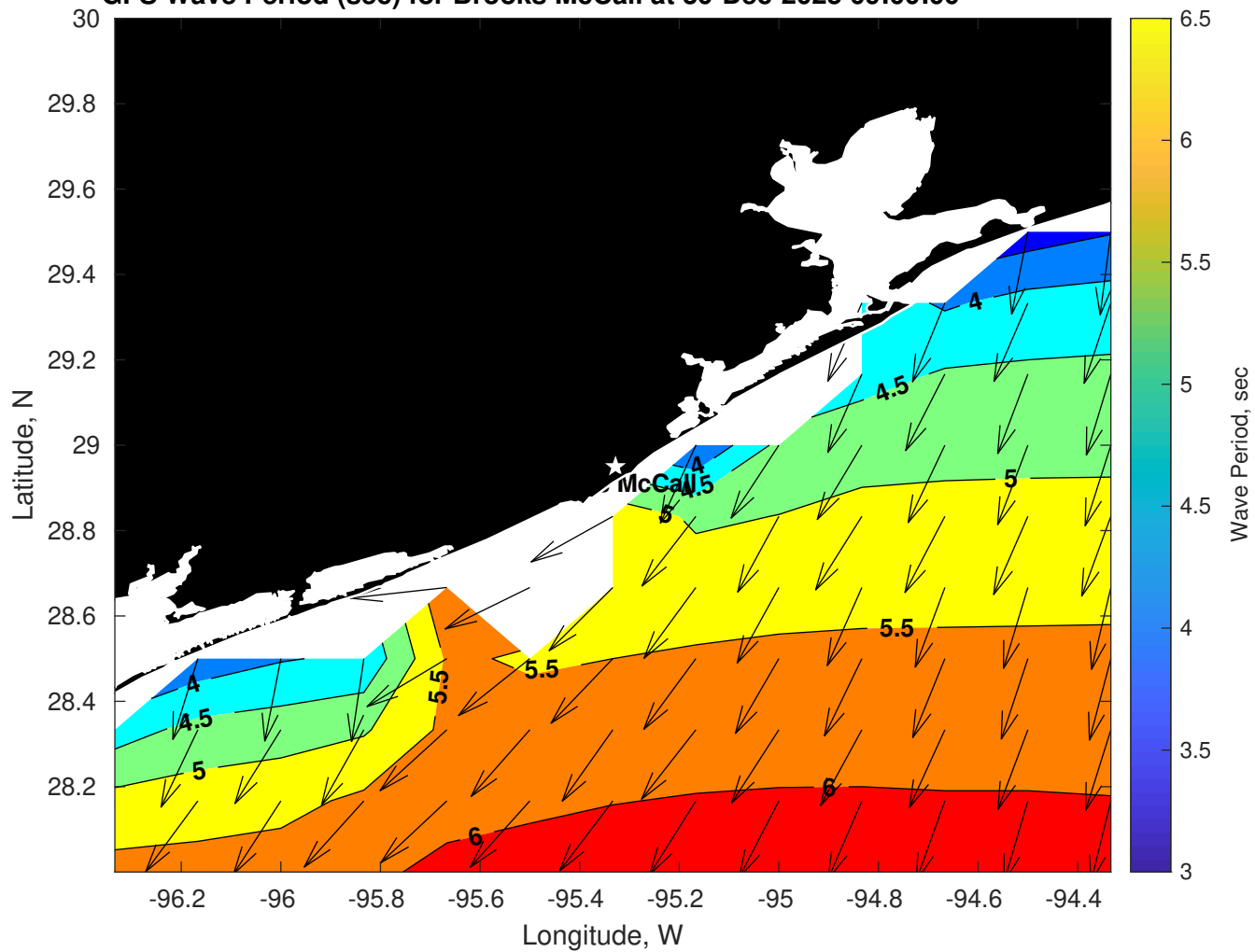
GFS Wave Period (sec) for Brooks McCall at 30-Dec-2025 09:00:00
