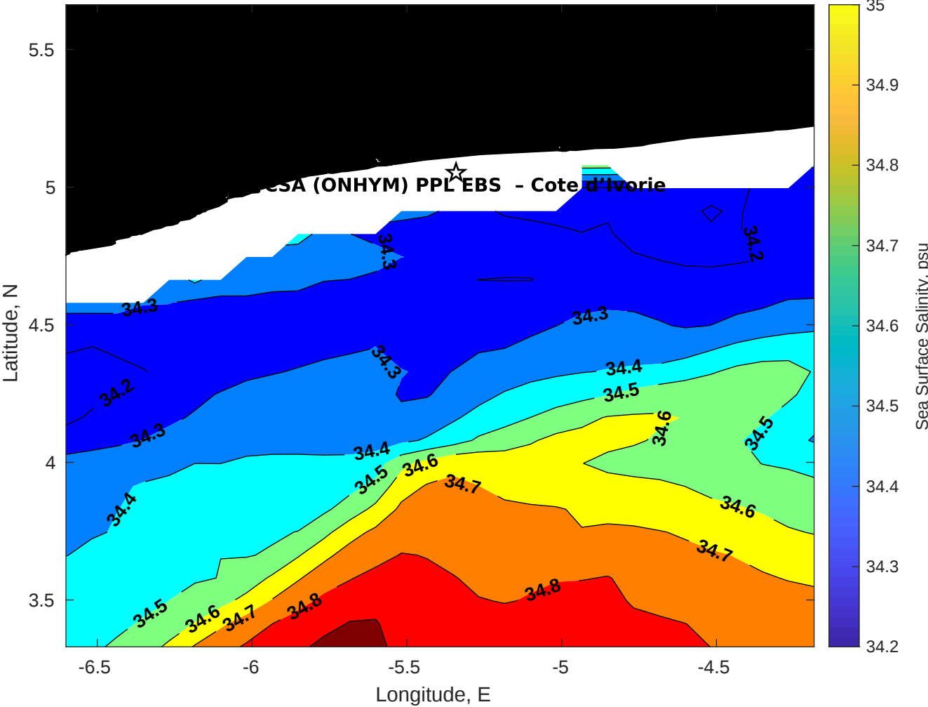
Surface Salinity for CSA (ONHYM) PPL EBS - Cote d'Ivoire at 29-Dec-2025 00:00:00
