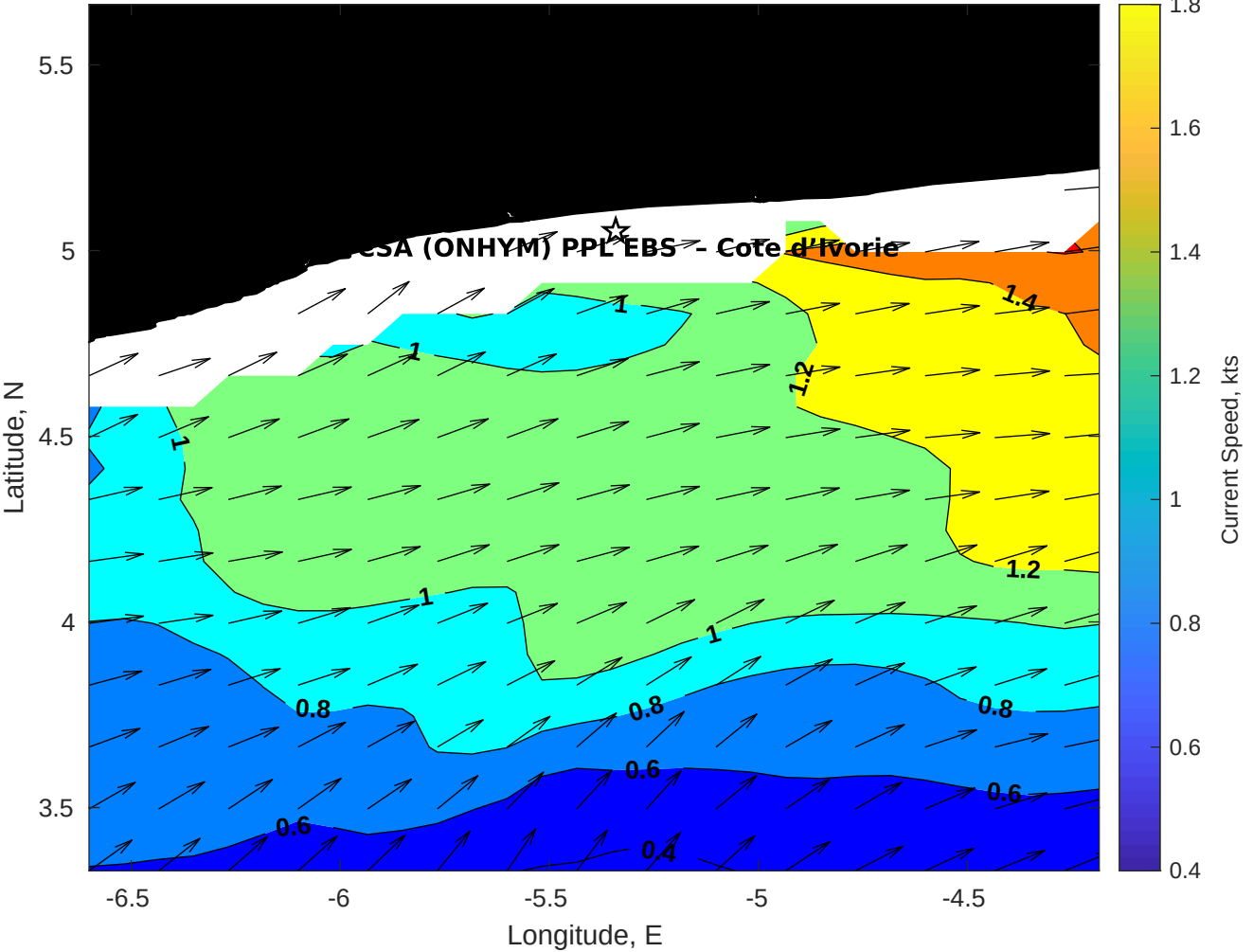
Surface Currents for CSA (ONHYM) PPL EBS - Cote d'Ivoire at 29-Dec-2025 00:00:00
