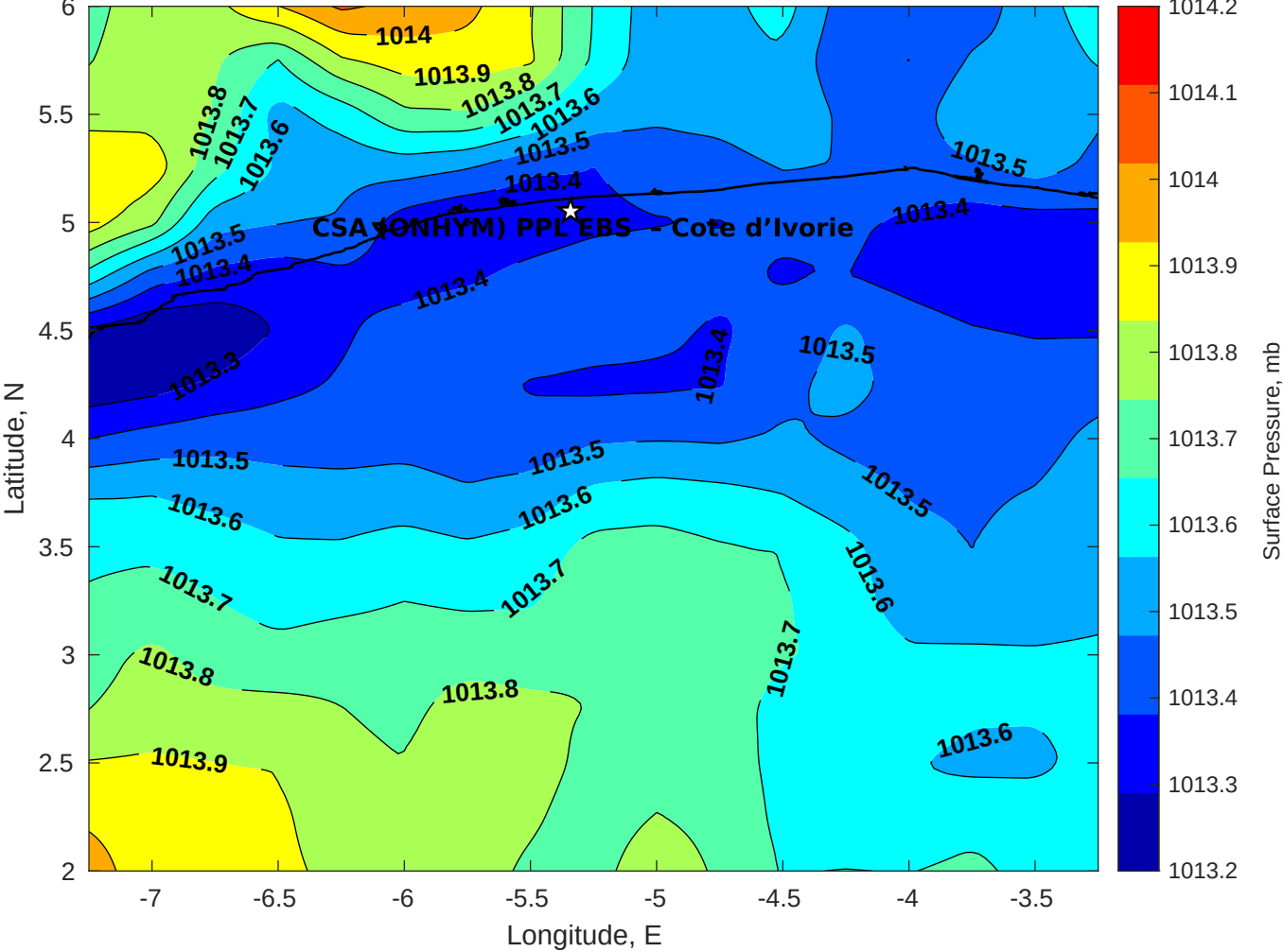
Surface Pressure (mb) for CSA (ONHYM) PPL EBS - Cote d'Ivoire at 31-Dec-2025 00:00:00
