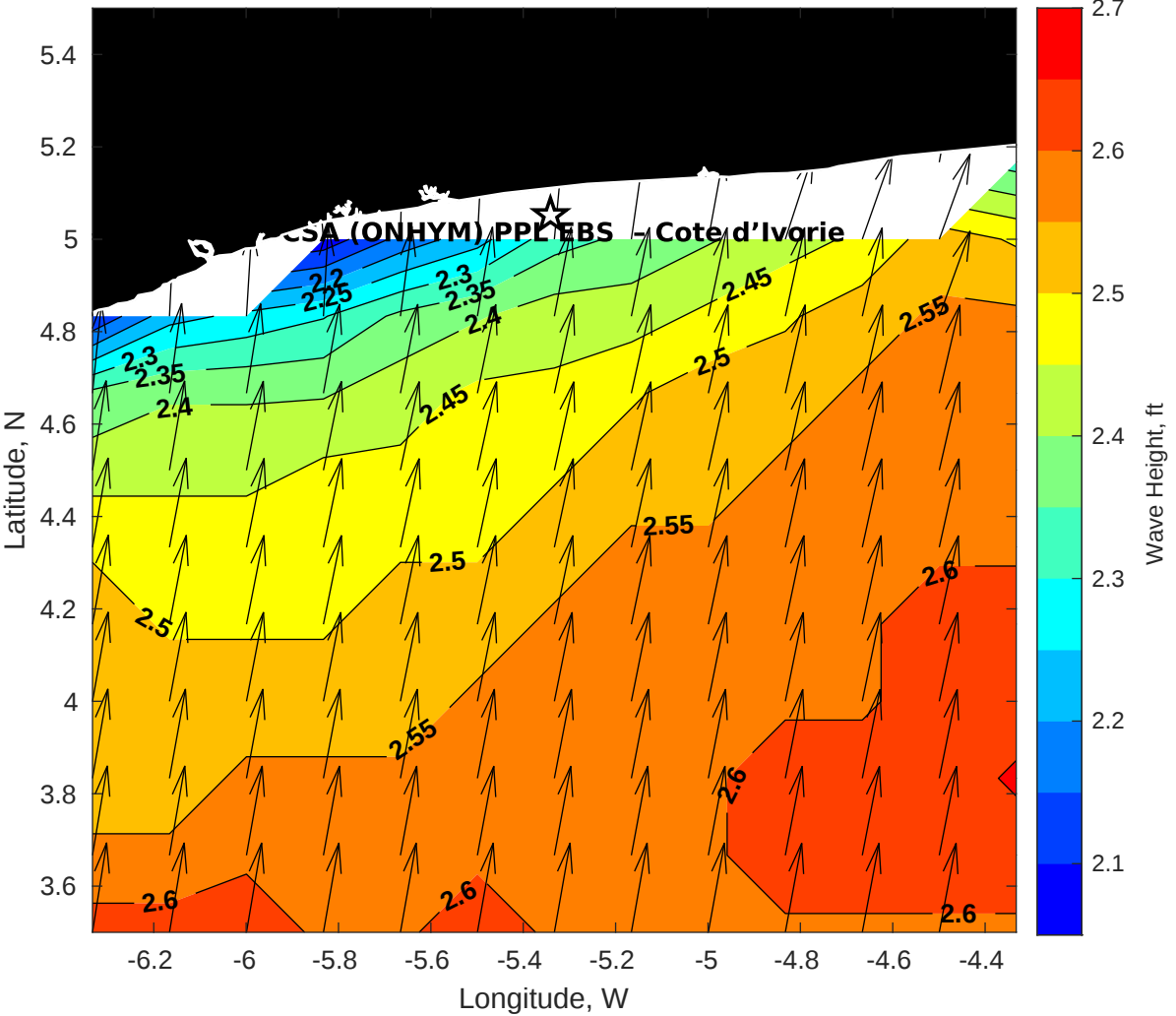
GFS Wave Height (ft) for CSA (ONHYM) PPL EBS - Cote d'Ivoire at 30-Dec-2025 09:00:00
