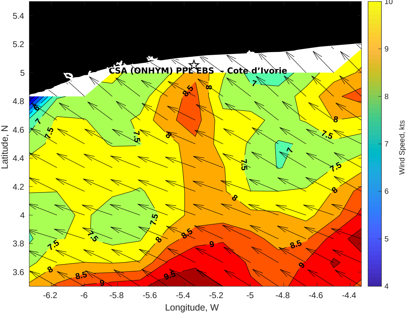
GFS Winds (kts) for CSA (ONHYM) PPL EBS - Cote d'Ivoire at 30-Dec-2025 09:00:00
