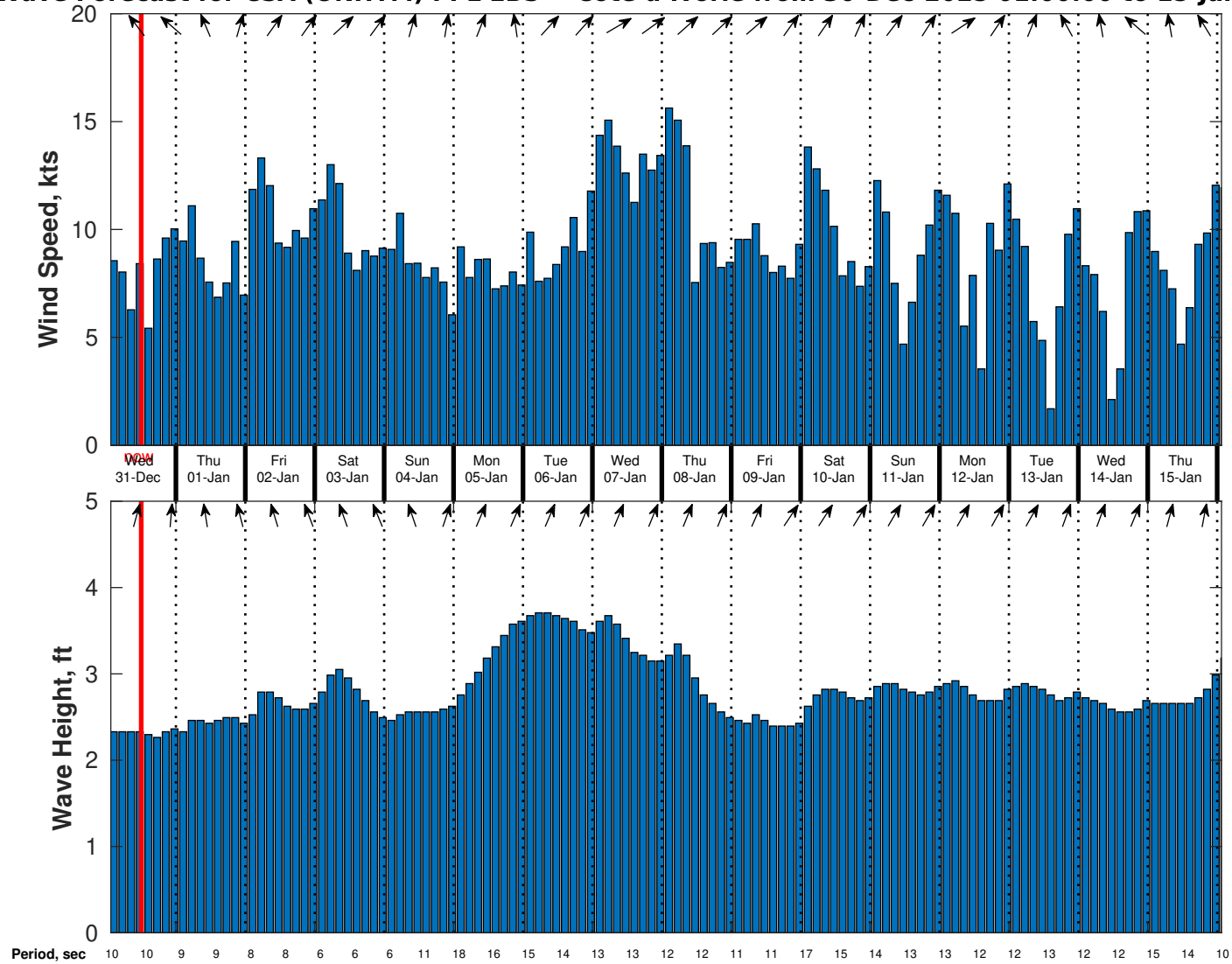
Wind & Wave Forecast for CSA (ONHYM) PPL EBS - Cote d'Ivoire from 30-Dec-2025 01:00:00 to 15-Jan-2026 01:00:00
