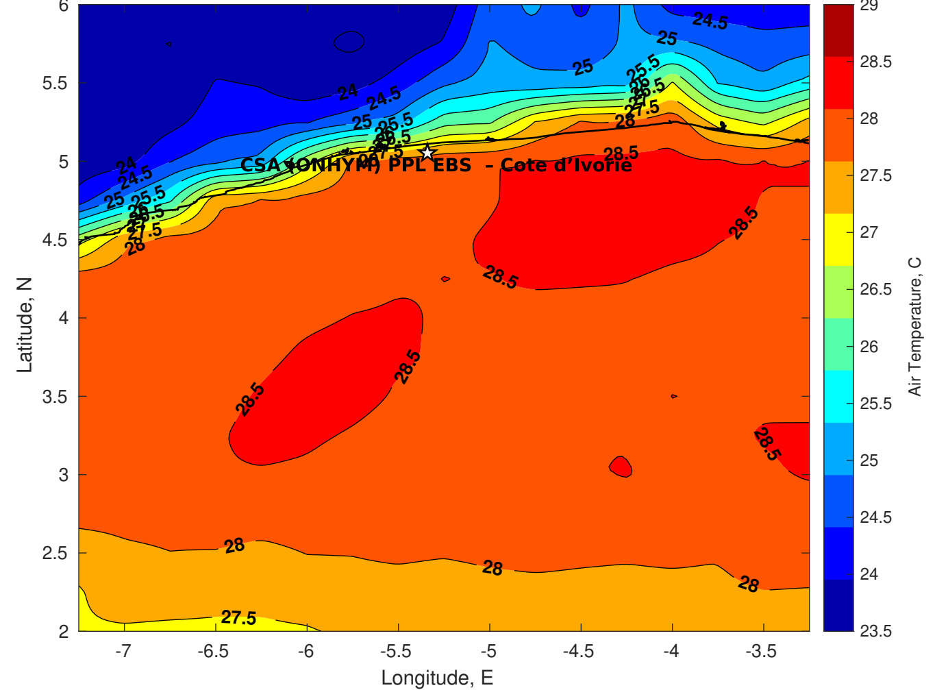
Air Temperature (C) for CSA (ONHYM) PPL EBS - Cote d'Ivoire at 30-Dec-2025
