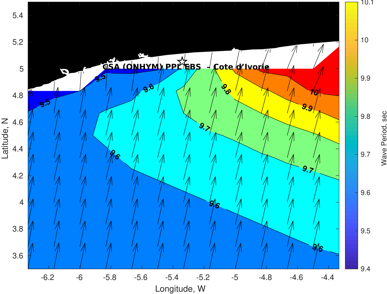
GFS Wave Period (sec) for CSA (ONHYM) PPL EBS - Cote d'Ivoire at 30-Dec-2025 09:00:00
