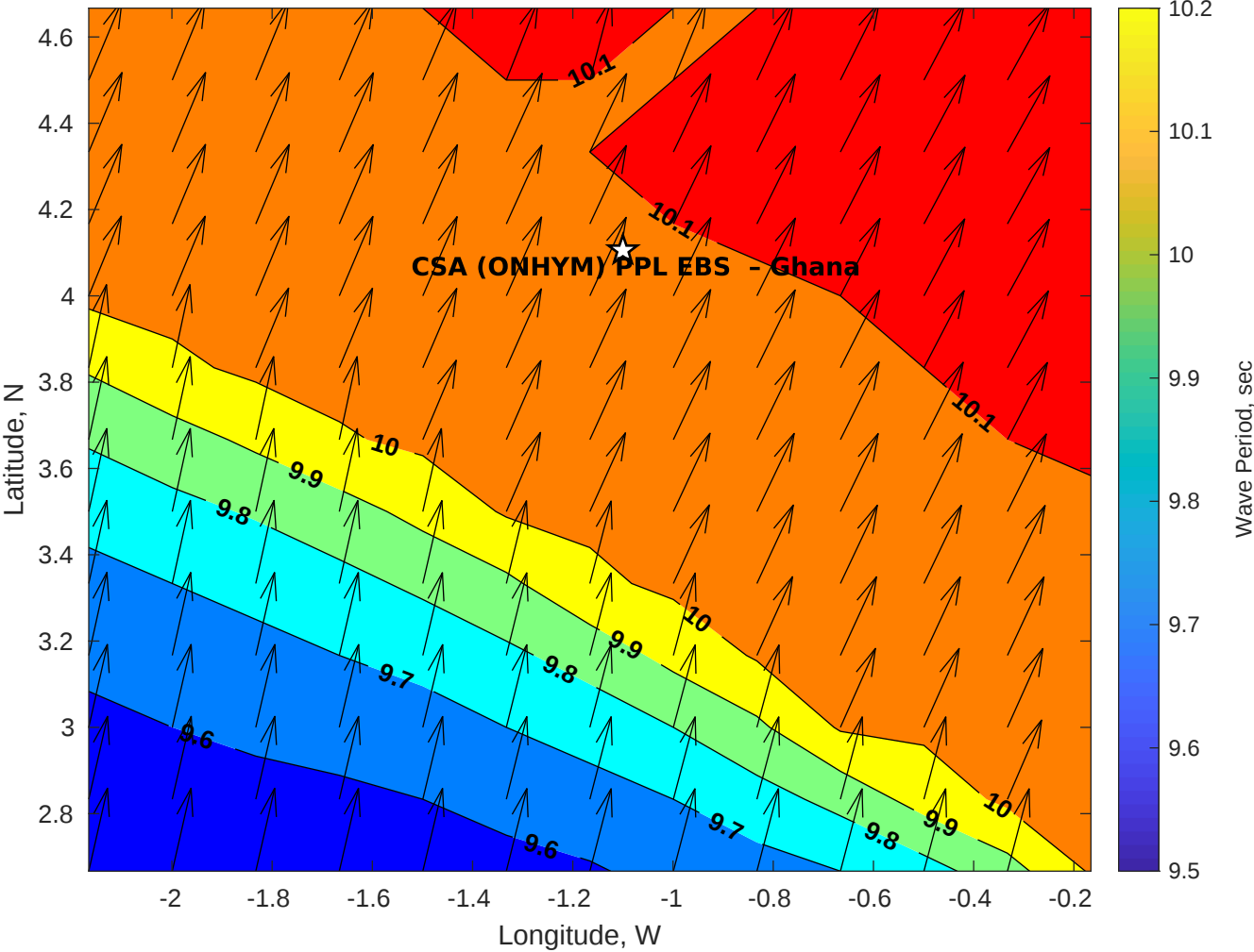
GFS Wave Period (sec) for CSA (ONHYM) PPL EBS - Ghana at 30-Dec-2025 09:00:00
