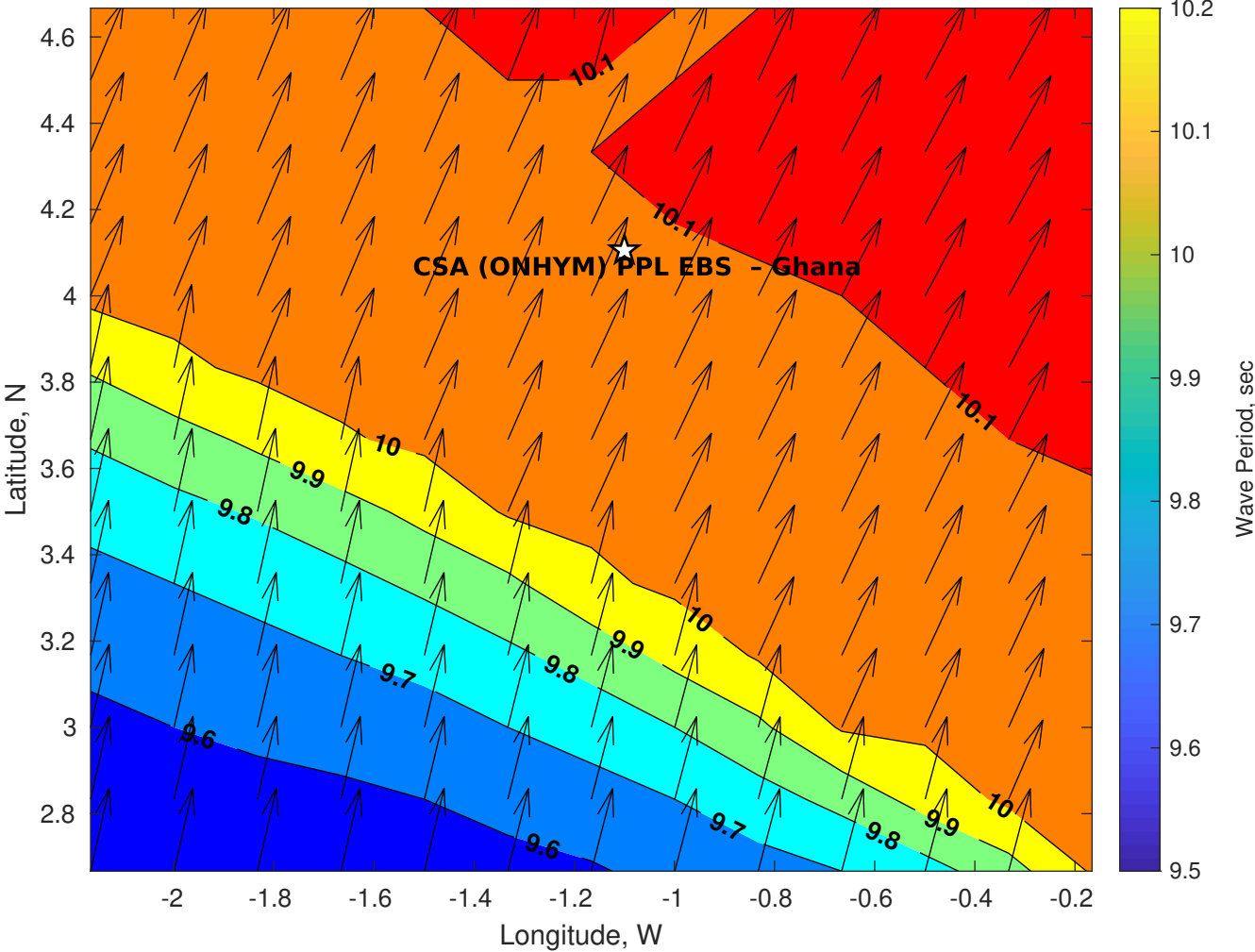
GFS Wave Period (sec) for CSA (ONHYM) PPL EBS - Ghana at 30-Dec-2025 09:00:00
