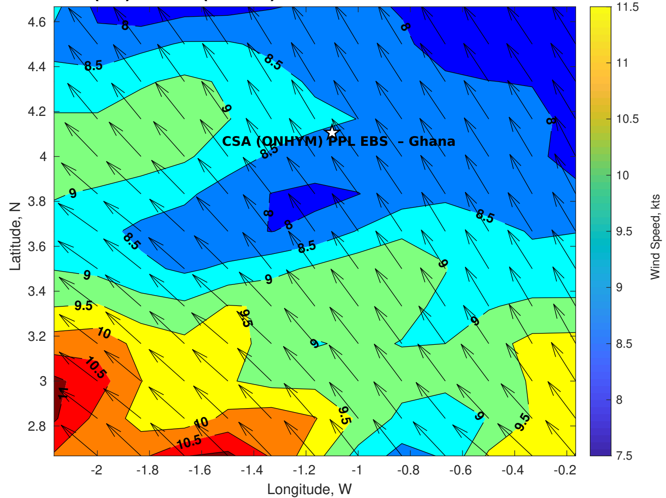
GFS Winds (kts) for CSA (ONHYM) PPL EBS - Ghana at 30-Dec-2025 09:00:00
