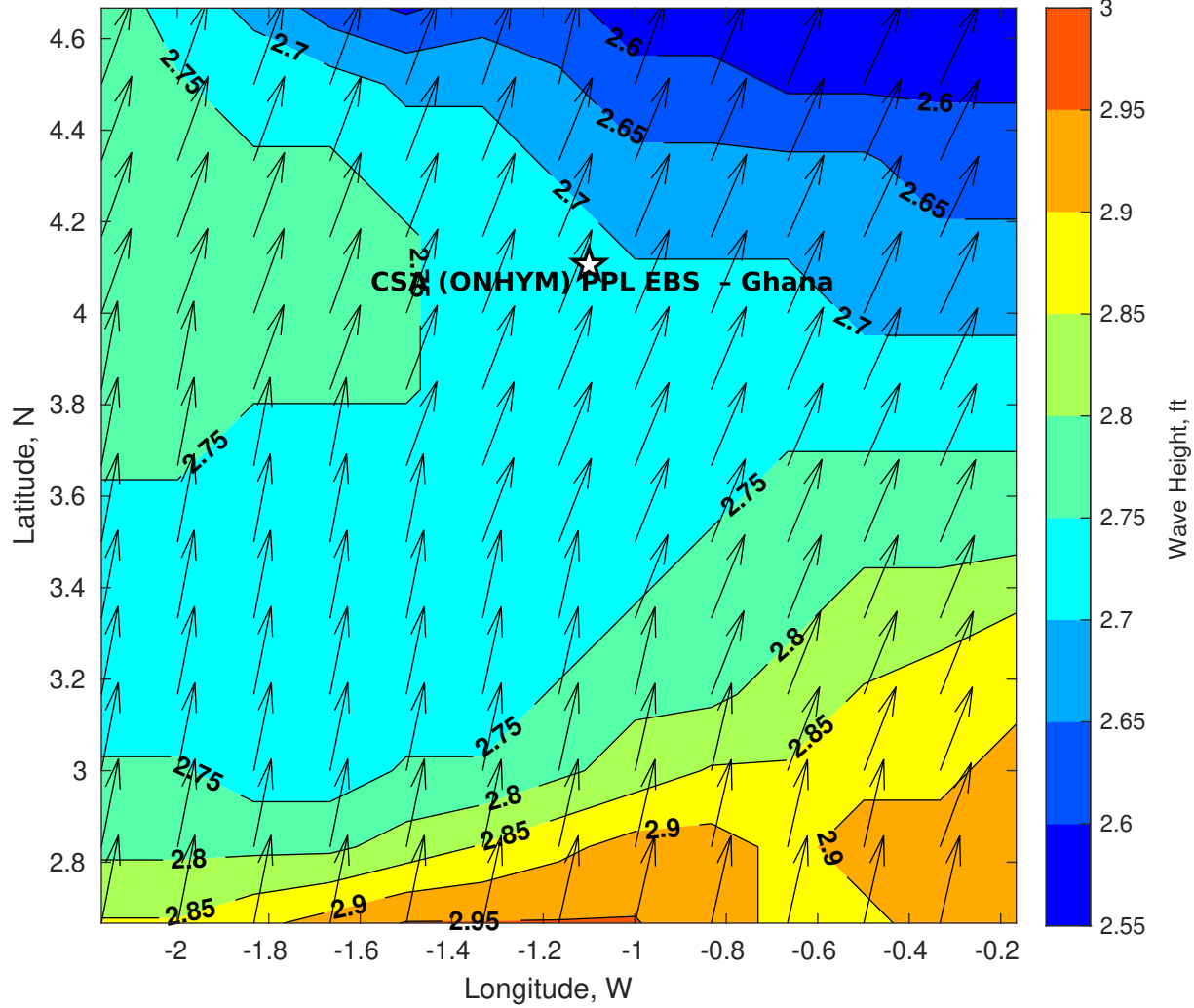
GFS Wave Height (ft) for CSA (ONHYM) PPL EBS - Ghana at 30-Dec-2025 09:00:00
