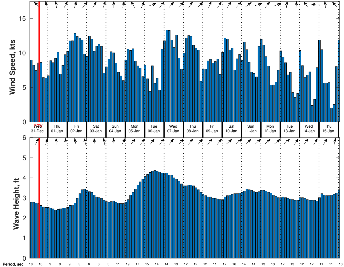
Wind & Wave Forecast for CSA (ONHYM) PPL EBS - Ghana from 30-Dec-2025 02:00:00 to 15-Jan-2026 02:00:00
