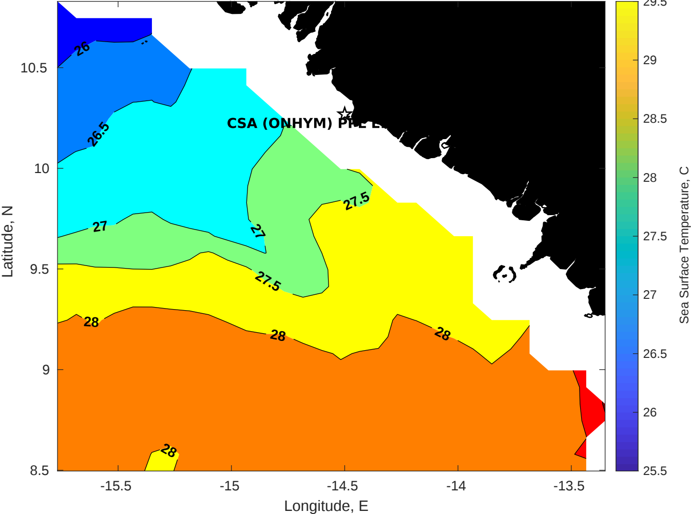
SST for CSA (ONHYM) PPL EBS - Guinea at 29-Dec-2025 00:00:00
