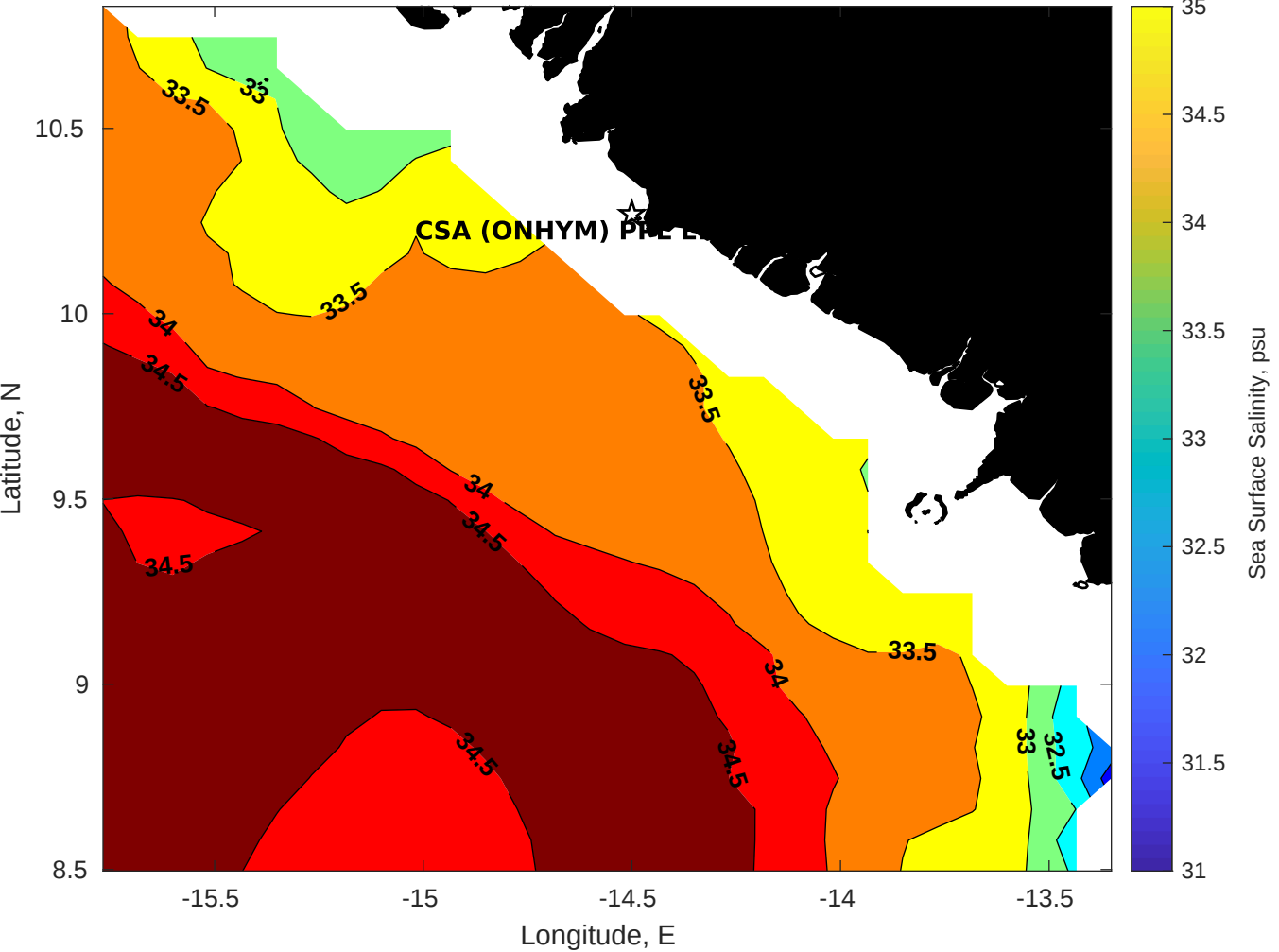
Surface Salinity for CSA (ONHYM) PPL EBS - Guinea at 29-Dec-2025 00:00:00
