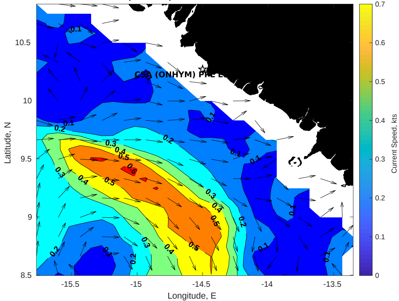
Surface Currents for CSA (ONHYM) PPL EBS - Guinea at 29-Dec-2025 00:00:00
