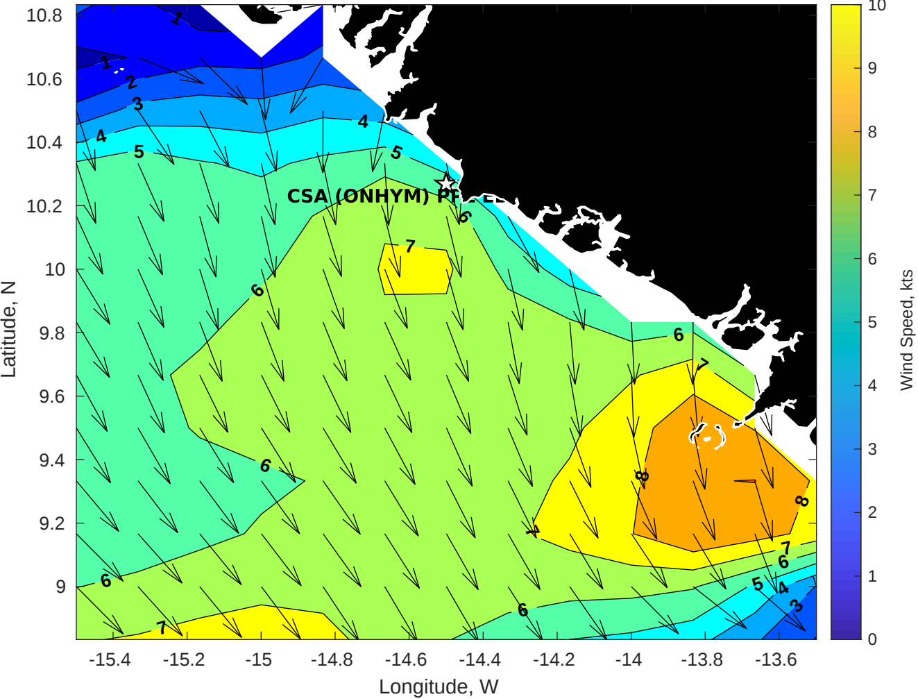
GFS Winds (kts) for CSA (ONHYM) PPL EBS - Guinea at 30-Dec-2025 09:00:00
