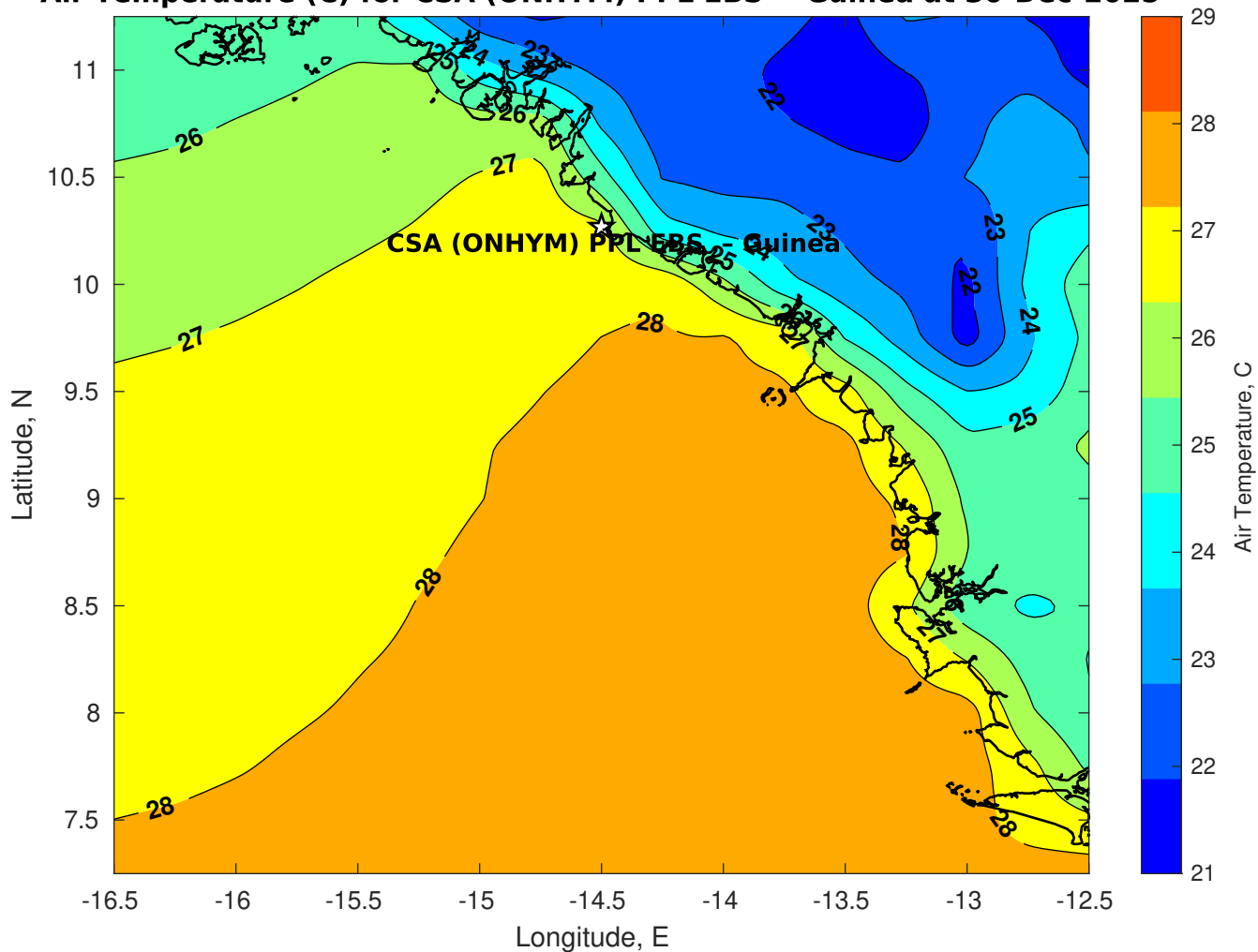
Air Temperature (C) for CSA (ONHYM) PPL EBS - Guinea at 30-Dec-2025
