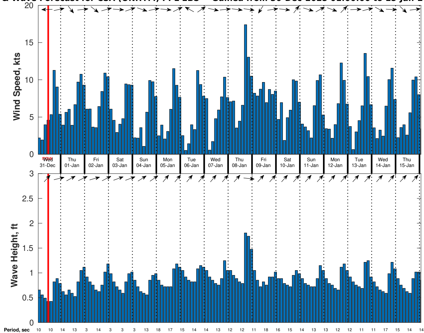
Wind & Wave Forecast for CSA (ONHYM) PPL EBS - Guinea from 30-Dec-2025 01:00:00 to 15-Jan-2026 01:00:00
