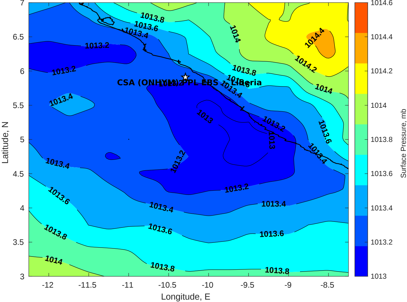
Surface Pressure (mb) for CSA (ONHYM) PPL EBS - Liberia at 31-Dec-2025 00:00:00
