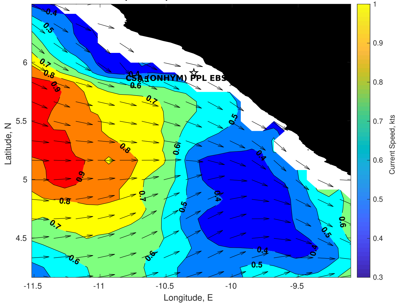
Surface Currents for CSA (ONHYM) PPL EBS - Liberia at 29-Dec-2025 00:00:00
