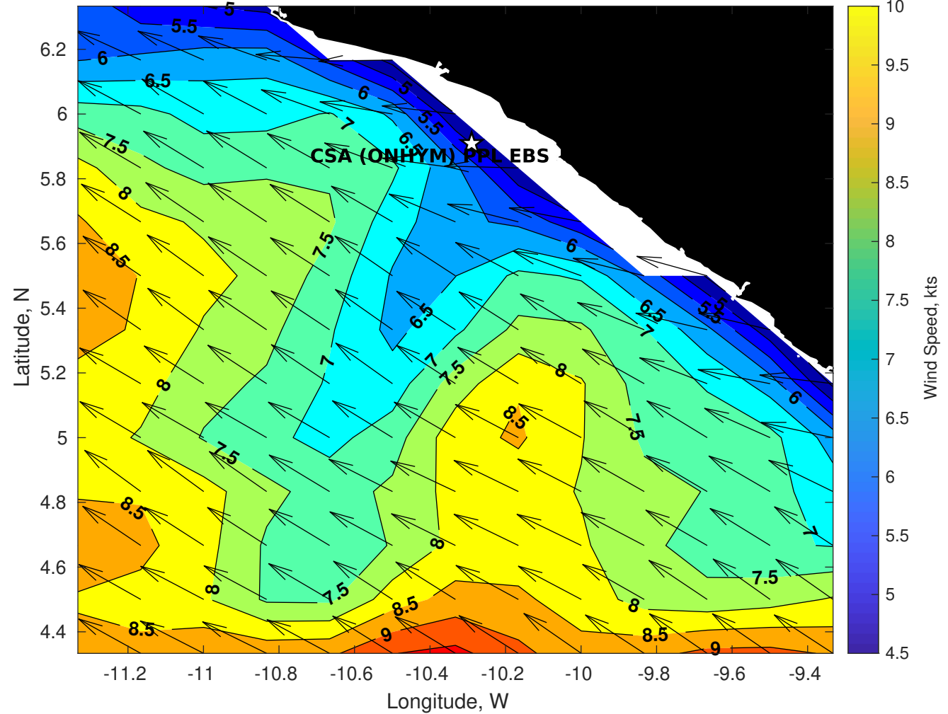
GFS Winds (kts) for CSA (ONHYM) PPL EBS - Liberia at 30-Dec-2025 09:00:00
