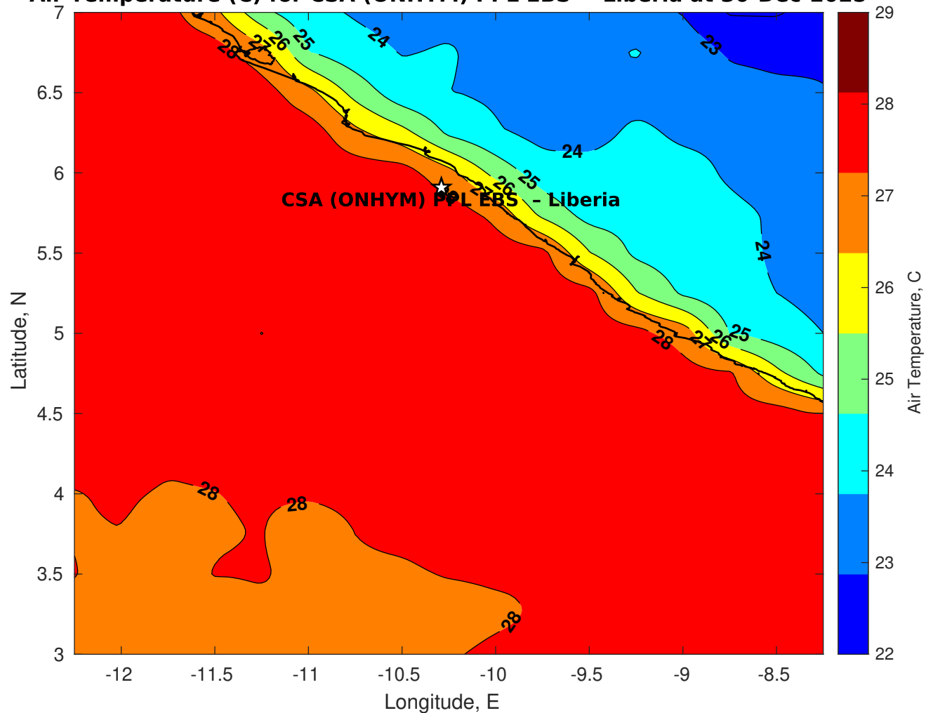
Air Temperature (C) for CSA (ONHYM) PPL EBS - Liberia at 30-Dec-2025
