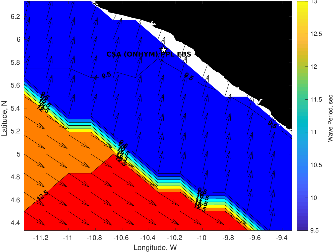
GFS Wave Period (sec) for CSA (ONHYM) PPL EBS - Liberia at 30-Dec-2025 09:00:00
