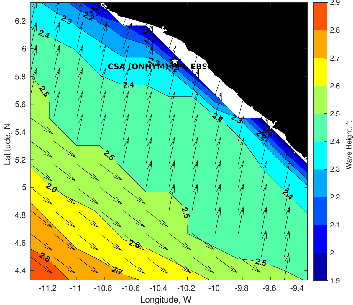
GFS Wave Height (ft) for CSA (ONHYM) PPL EBS - Liberia at 30-Dec-2025 09:00:00
