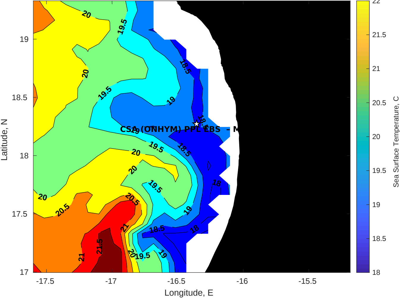
SST for CSA (ONHYM) PPL EBS - Mauritania at 29-Dec-2025 00:00:00
