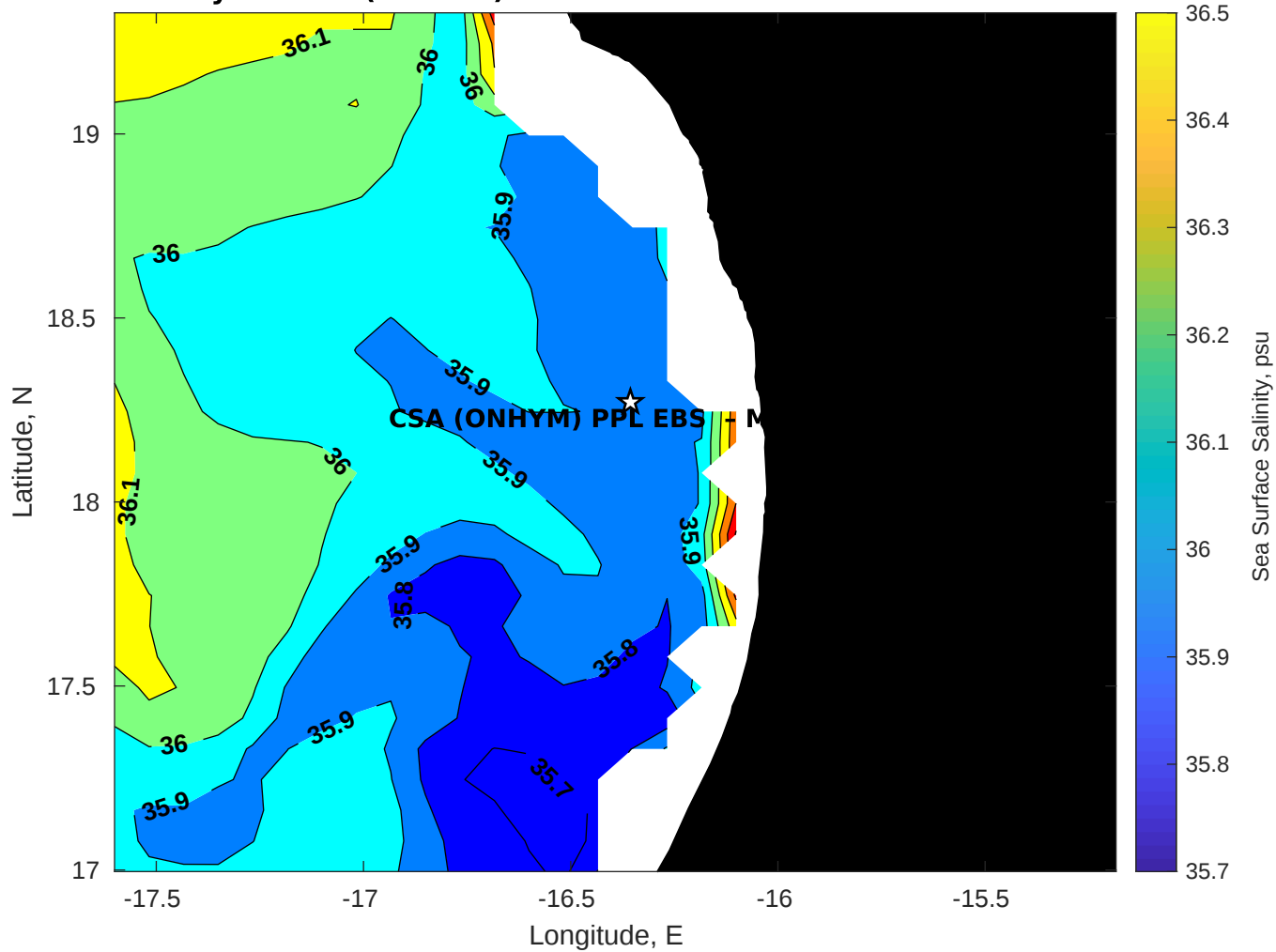
Surface Salinity for CSA (ONHYM) PPL EBS - Mauritania at 29-Dec-2025 00:00:00
