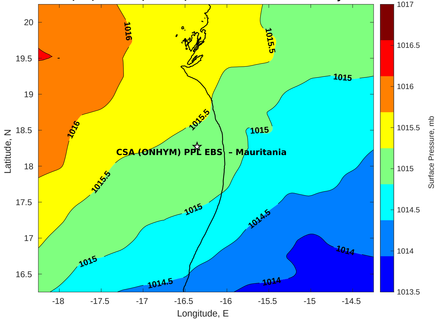
Surface Pressure (mb) for CSA (ONHYM) PPL EBS - Mauritania at 01-Jan-2026 00:00:00
