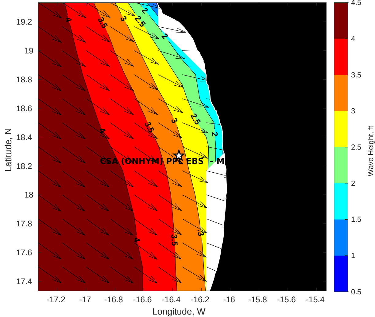
GFS Wave Height (ft) for CSA (ONHYM) PPL EBS - Mauritania at 30-Dec-2025 09:00:00
