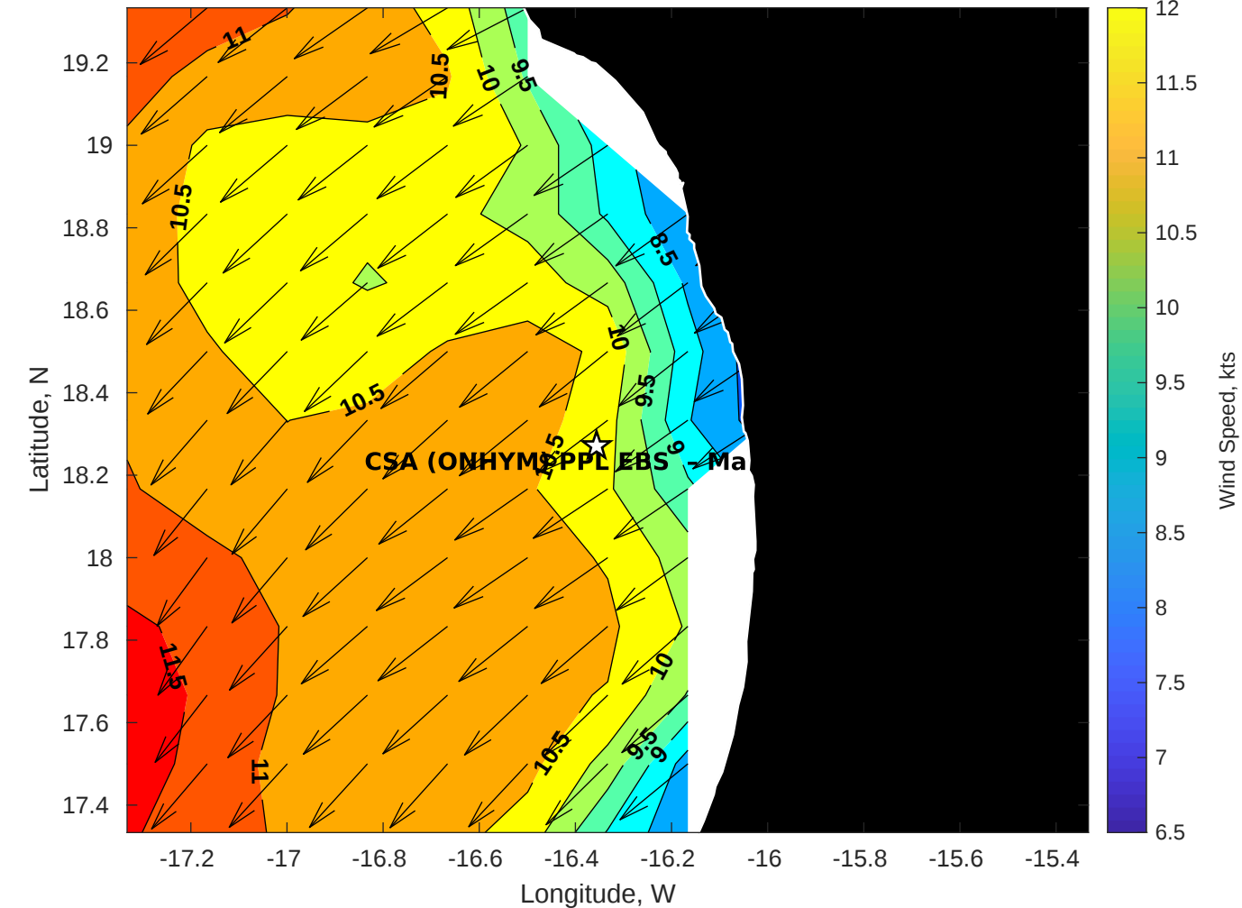
GFS Winds (kts) for CSA (ONHYM) PPL EBS - Mauritania at 30-Dec-2025 09:00:00
