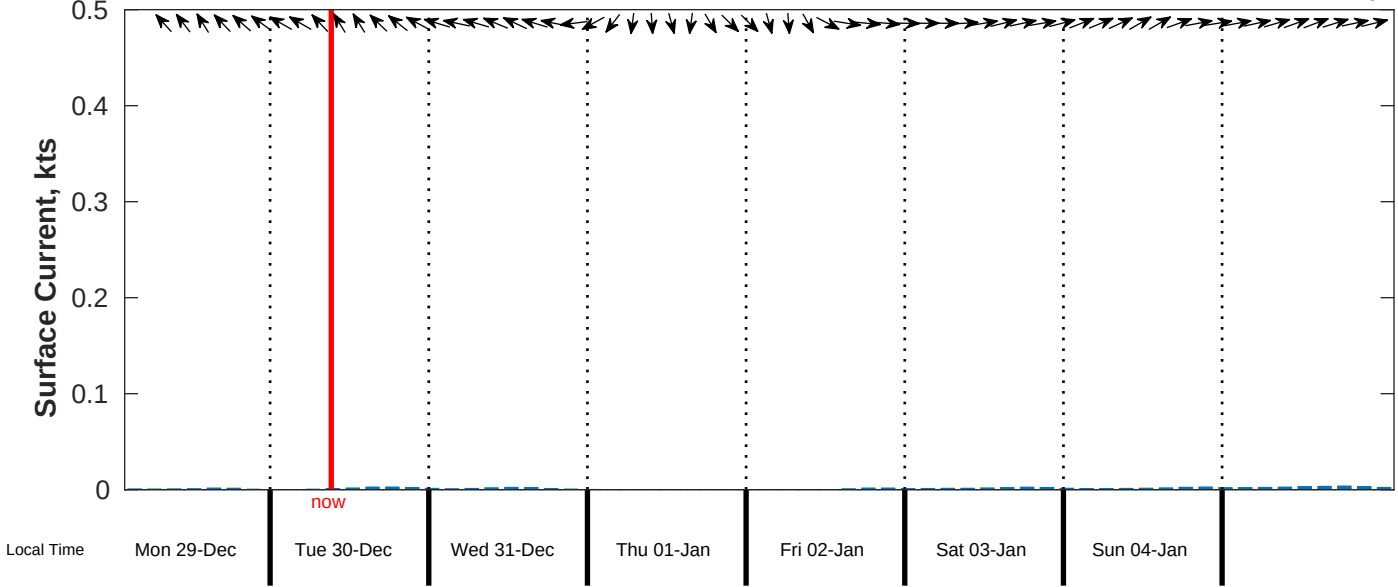
Surface Current Forecast for CSA (ONHYM) PPL EBS - Mauritania from 29-Dec-2025 00:00:00 to 06-Jan-2026 00:00:00
