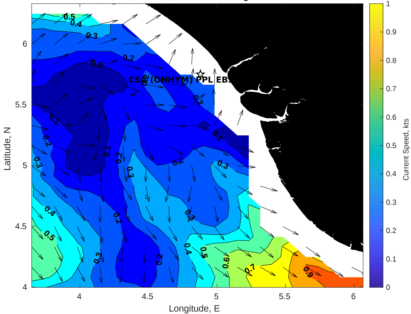
Surface Currents for CSA (ONHYM) PPL EBS - Nigeria at 29-Dec-2025 00:00:00
