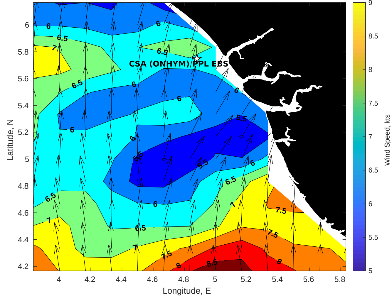
GFS Winds (kts) for CSA (ONHYM) PPL EBS - Nigeria at 30-Dec-2025 09:00:00
