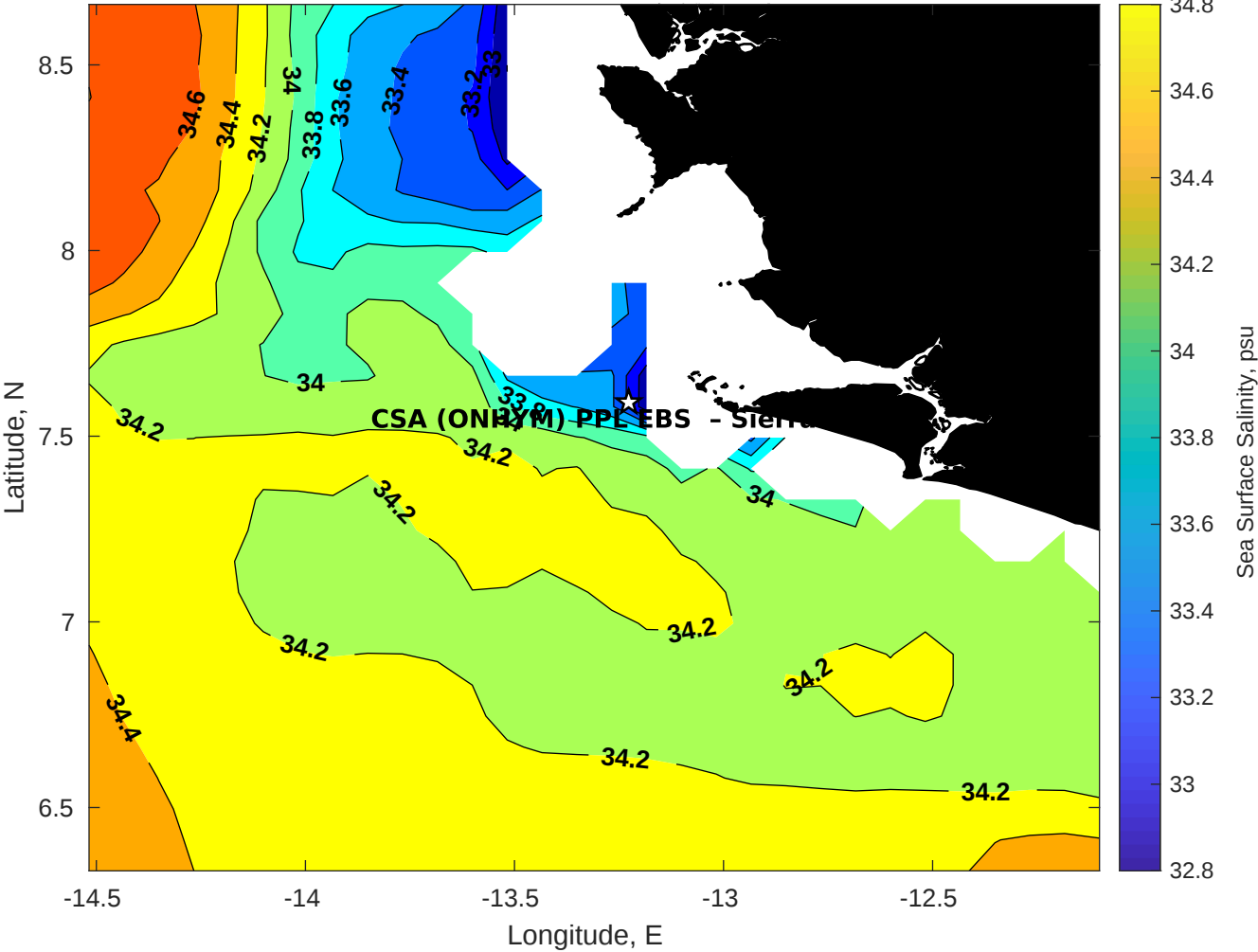
Surface Salinity for CSA (ONHYM) PPL EBS - Sierra Leone at 29-Dec-2025 00:00:00
