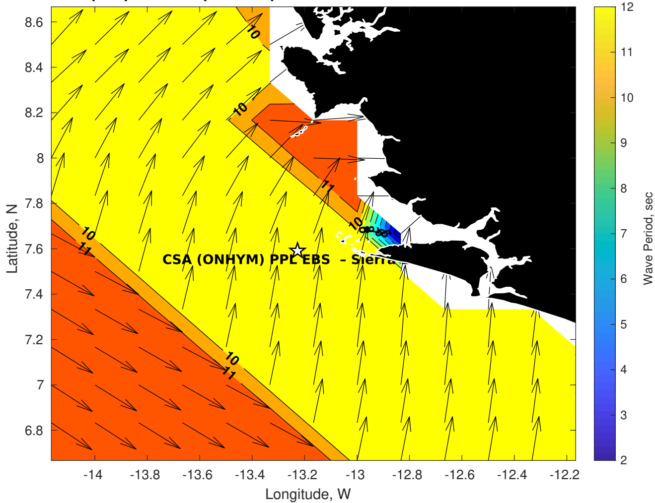
GFS Wave Period (sec) for CSA (ONHYM) PPL EBS - Sierra Leone at 30-Dec-2025 09:00:00
