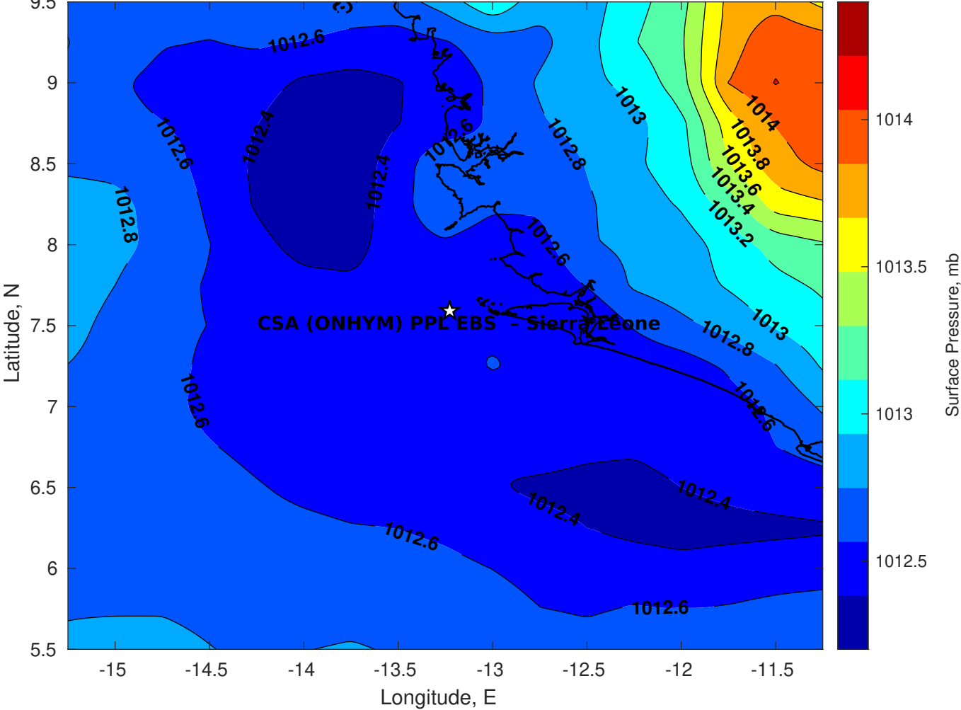
Surface Pressure (mb) for CSA (ONHYM) PPL EBS - Sierra Leone at 30-Dec-2025 00:00:00
