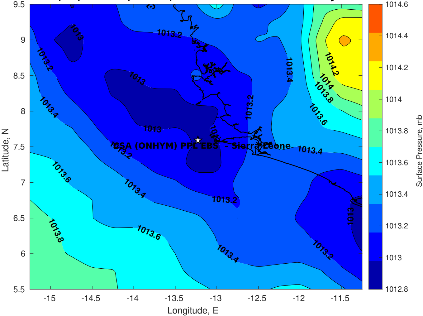
Surface Pressure (mb) for CSA (ONHYM) PPL EBS - Sierra Leone at 01-Jan-2026 00:00:00
