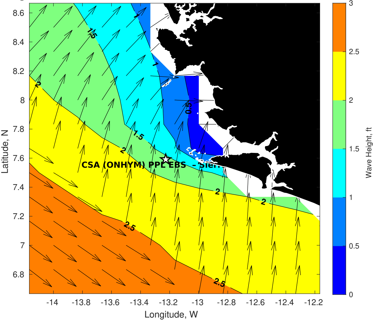
GFS Wave Height (ft) for CSA (ONHYM) PPL EBS - Sierra Leone at 30-Dec-2025 09:00:00
