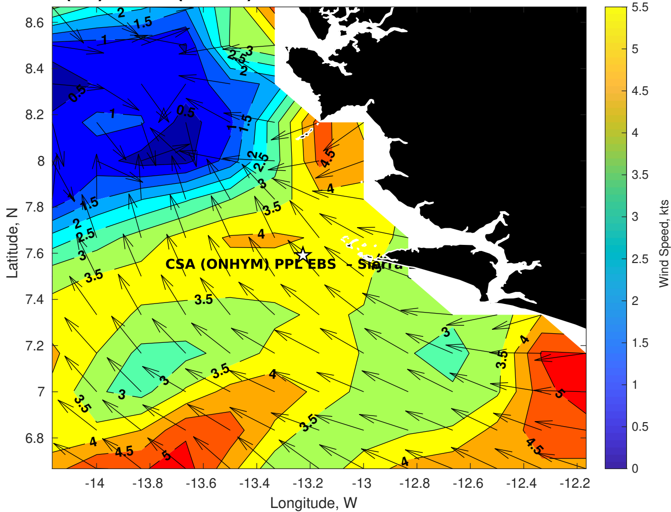
GFS Winds (kts) for CSA (ONHYM) PPL EBS - Sierra Leone at 30-Dec-2025 09:00:00
