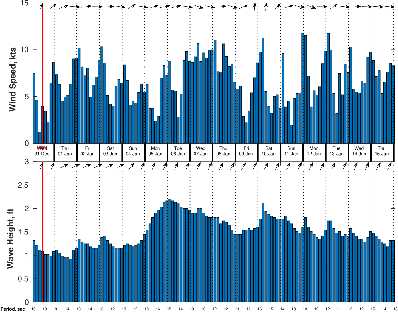
Wind & Wave Forecast for CSA (ONHYM) PPL EBS - Sierra Leone from 30-Dec-2025 01:00:00 to 15-Jan-2026 01:00:00
