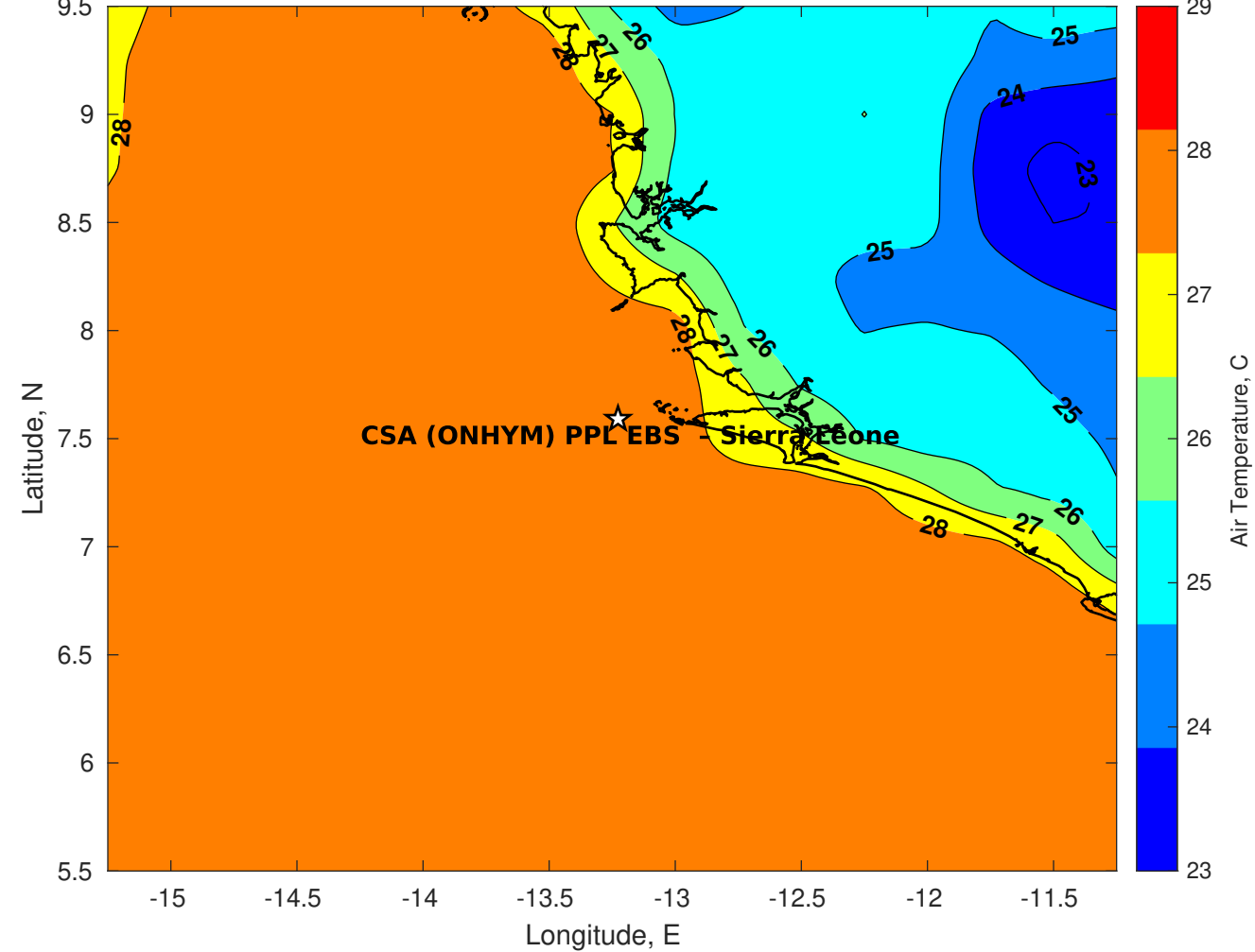
Air Temperature (C) for CSA (ONHYM) PPL EBS - Sierra Leone at 30-Dec-2025
