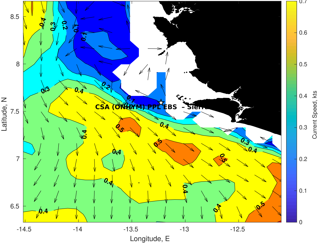
Surface Currents for CSA (ONHYM) PPL EBS - Sierra Leone at 29-Dec-2025 00:00:00
