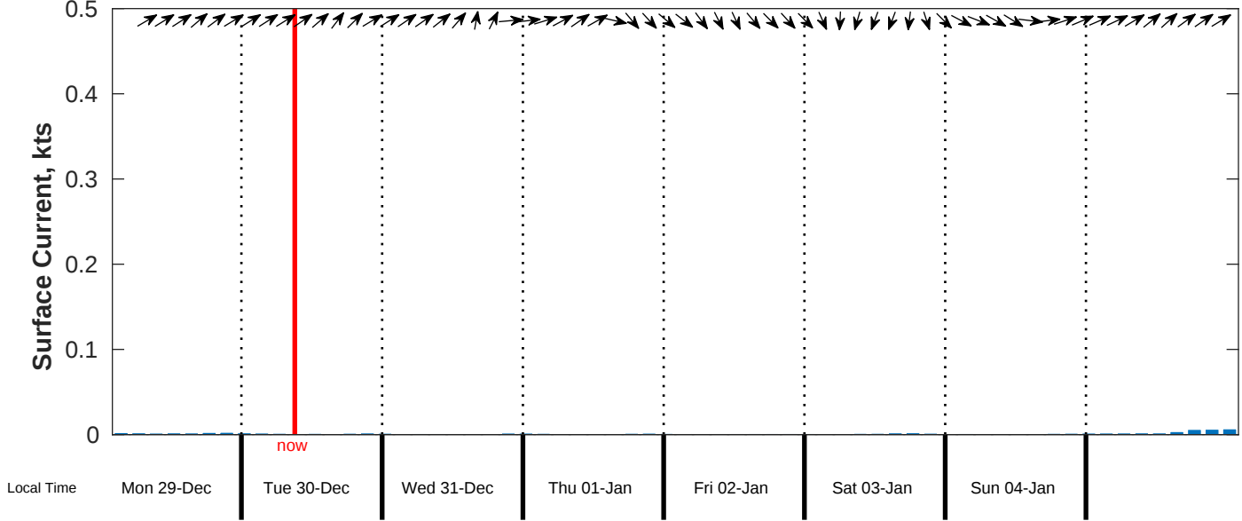
Surface Current Forecast for CSA (ONHYM) PPL EBS - Western Sahara from 29-Dec-2025 00:00:00 to 06-Jan-2026 00:00:00
