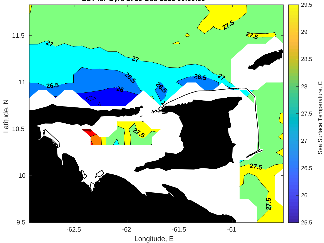
SST for Gyre at 29-Dec-2025 00:00:00
