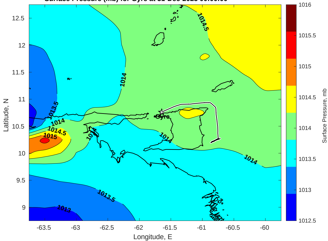
Surface Pressure (mb) for Gyre at 31-Dec-2025 00:00:00
