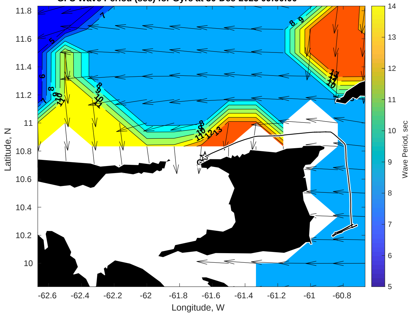
GFS Wave Period (sec) for Gyre at 30-Dec-2025 09:00:00
