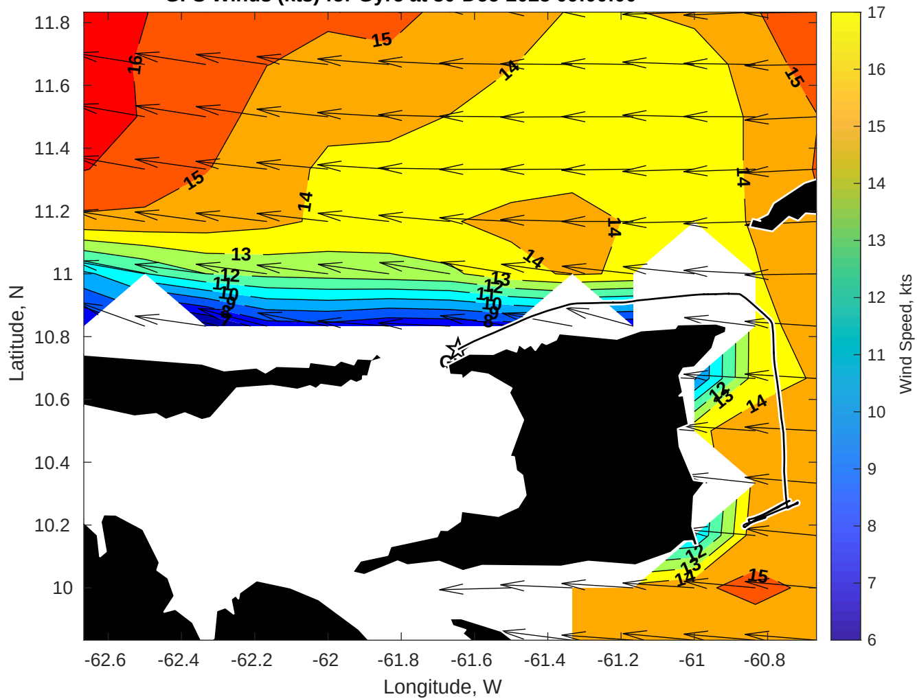
GFS Winds (kts) for Gyre at 30-Dec-2025 09:00:00
