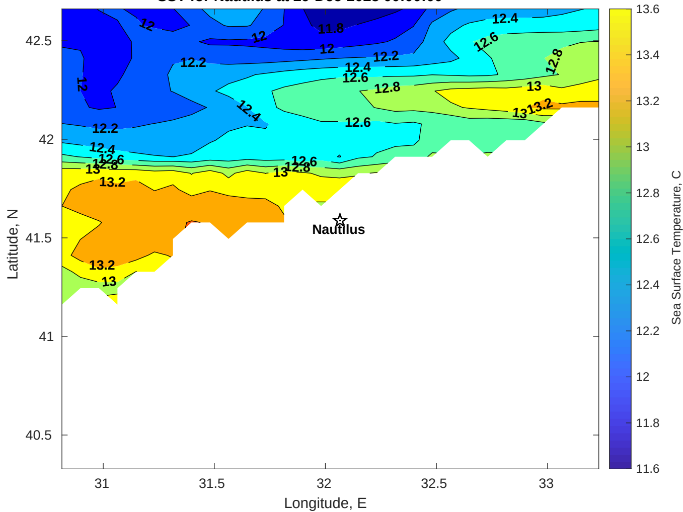
SST for Nautilus at 29-Dec-2025 00:00:00
