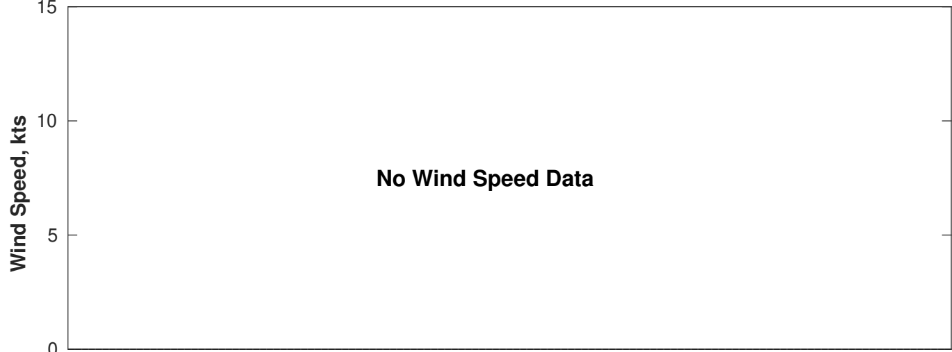
Wind & Wave Forecast for Nautilus from 30-Dec-2025 02:00:00 to 15-Jan-2026 02:00:00
