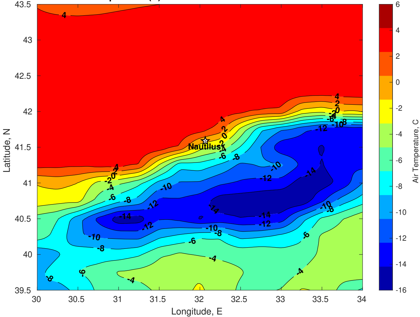
Air Temperature (C) for Nautilus at 30-Dec-2025
