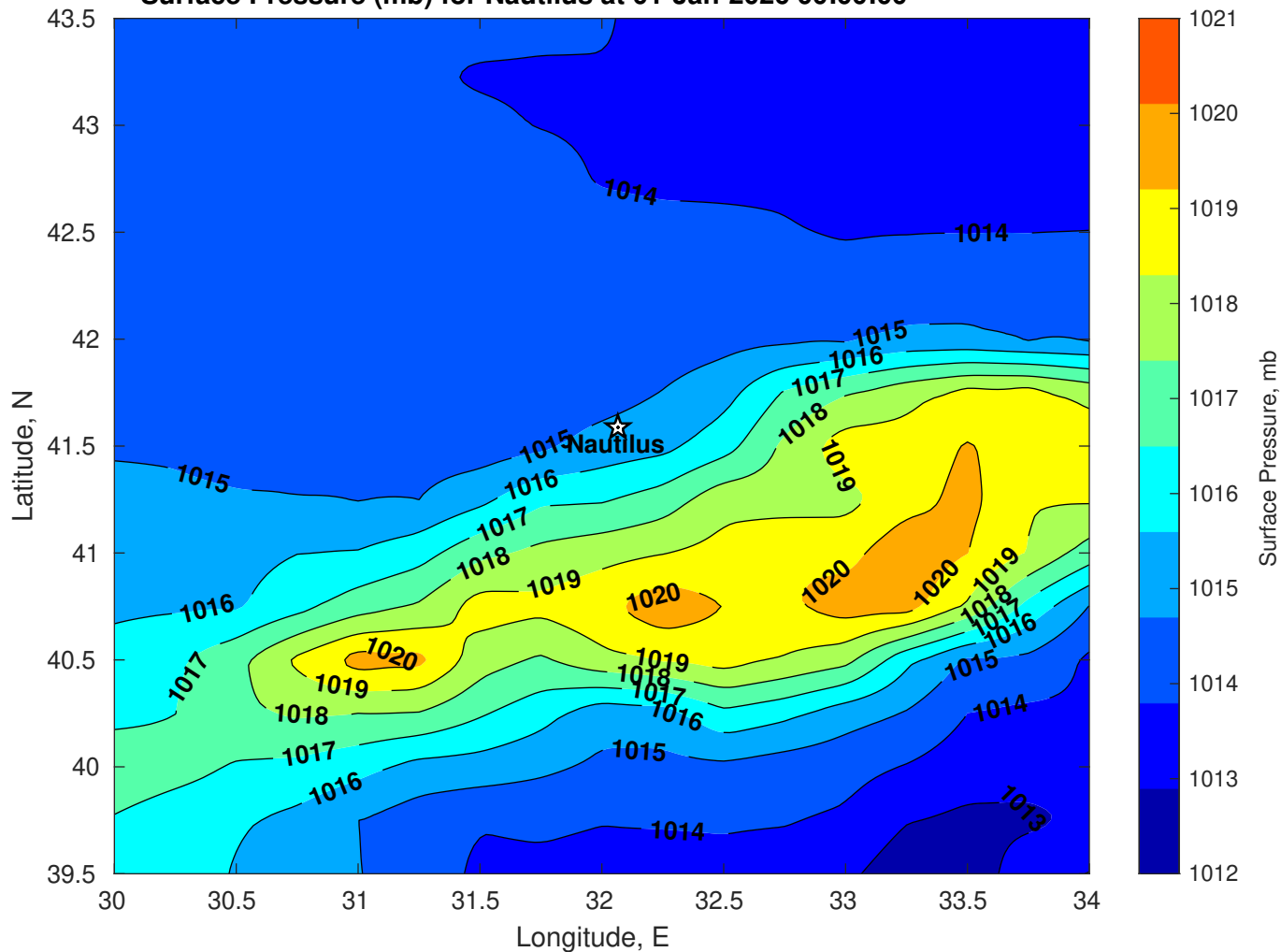
Surface Pressure (mb) for Nautilus at 01-Jan-2026 00:00:00
