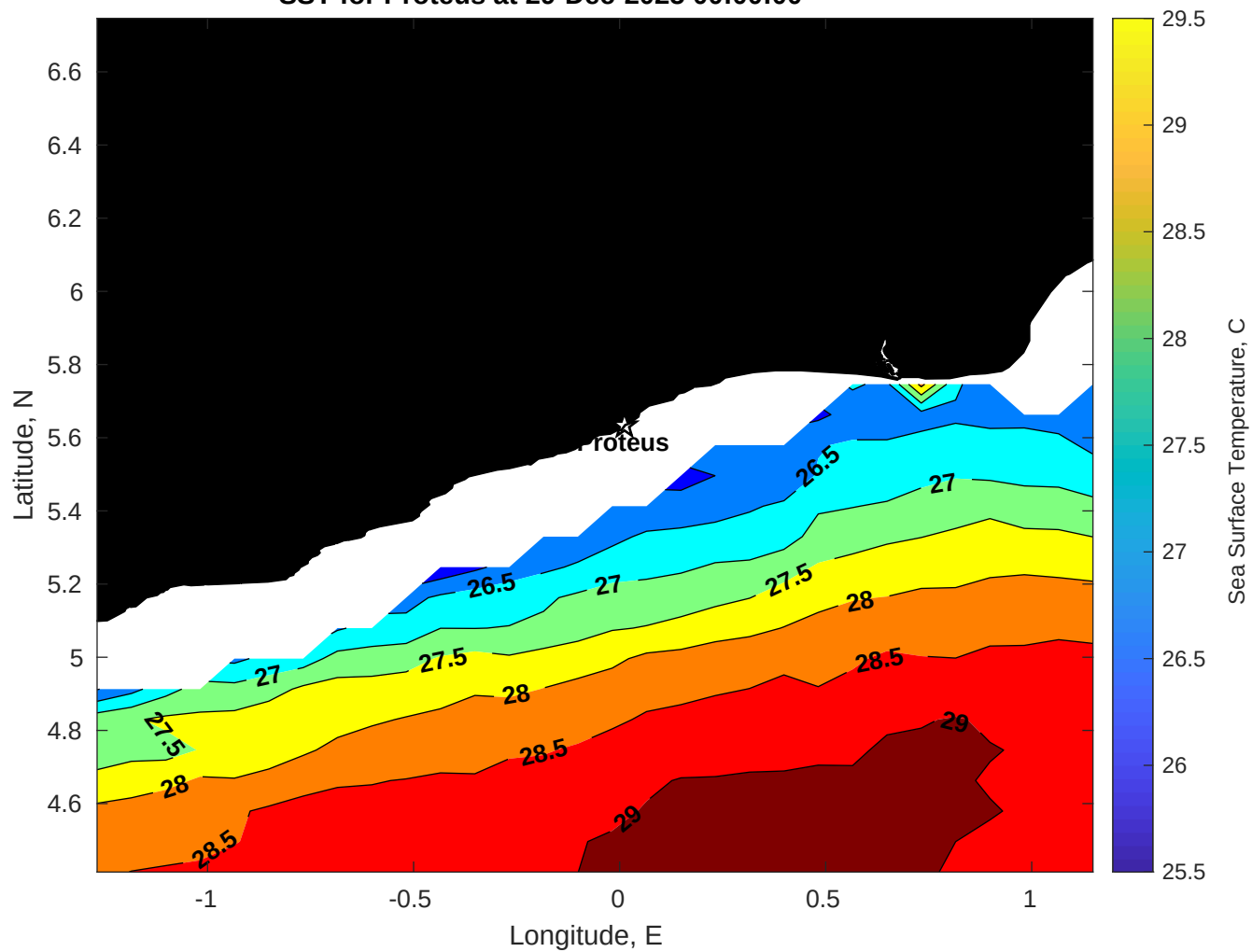
SST for Proteus at 29-Dec-2025 00:00:00
