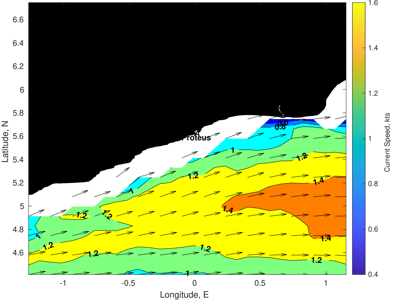
Surface Currents for Proteus at 29-Dec-2025 00:00:00
