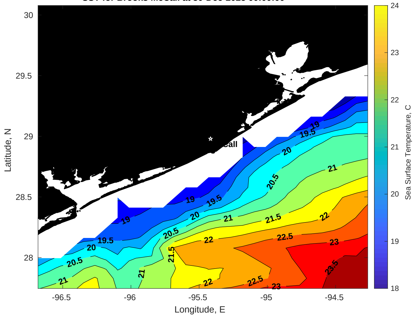
SST for Brooks McCall at 30-Dec-2025 00:00:00
